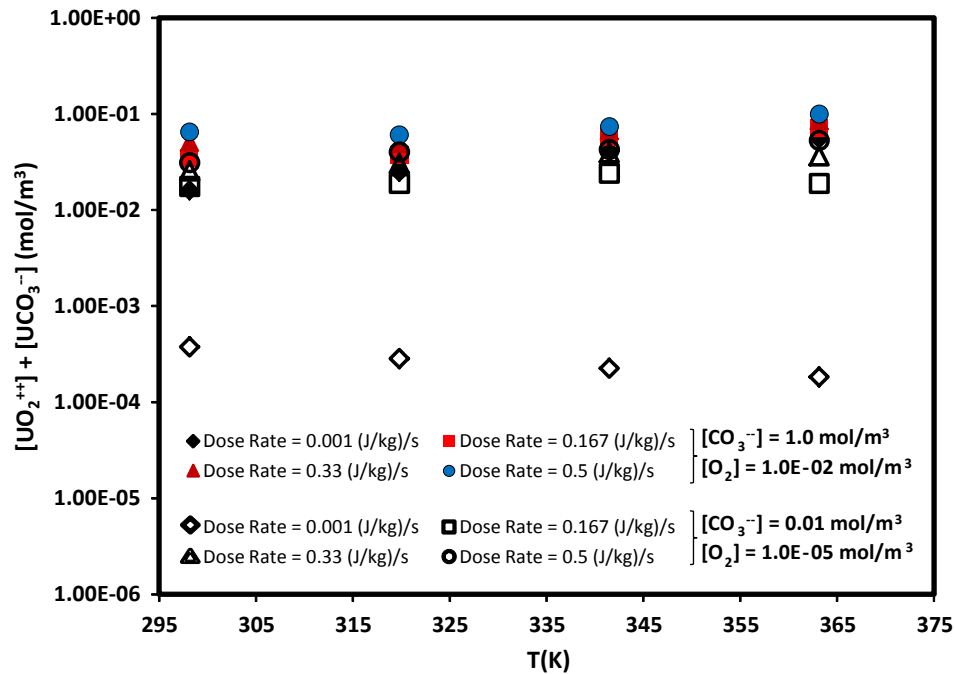
Figure 4.3. Concentration profile of U aqueous species computed by the MPM as a function of temperature, dose rate, CO_3^{2-} , and O_2 concentrations.
