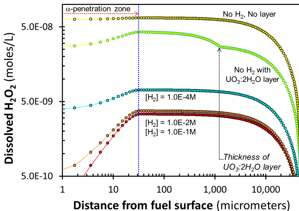
Figure 7.5. Concentration profiles of hydrogen peroxide produced by alpha radiolysis as a function of distance away from the fuel surface. Each point in the plot is an individual model realization in time and space.
