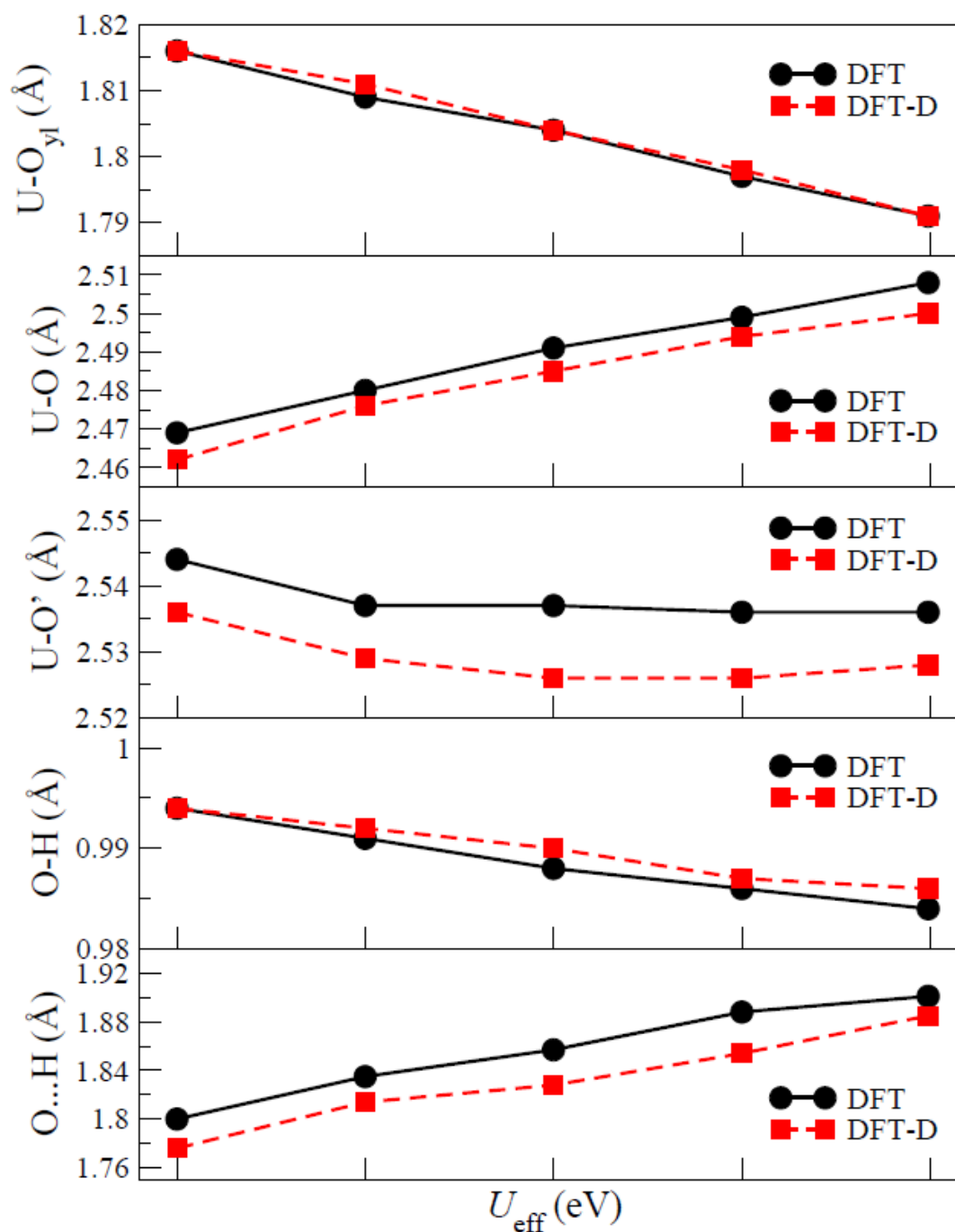
Figure 11.12. Evolution of the computed U–O, O–H and O··H bond distances in \alpha\text{-UO}_2(\text{OH})_2 , as functions of the effective Hubbard parameter, U_{\text{eff}} . Calculations were carried out at the GGA+ U /PBE level of theory, with (DFT-D) and without inclusion of dispersion corrections (DFT).
