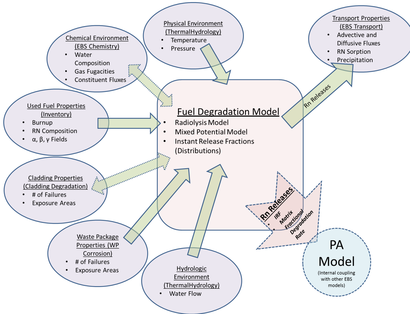
Figure 1.7. Schematic of potential parameter connections for fully embedded coupled fuel degradation model with a performance assessment (PA) model. Solid arrows unidirectional connections, whereas dotted arrows indicate bidirectional couplings between subsystem models within the PA model.
