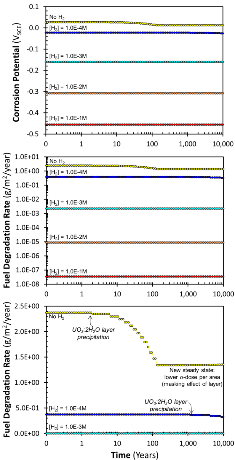
Figure 7.4. Examples of time-dependent fuel corrosion potentials and corresponding degradation rates calculated with the MPM for different dissolved hydrogen concentrations with 1% NMP at the fuel surface.
