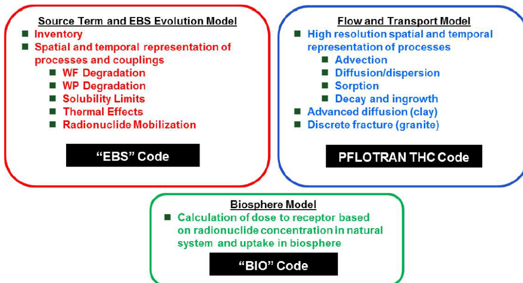
Figure 1.5. Disposal system integrated process models (Freeze et al. 2013).
