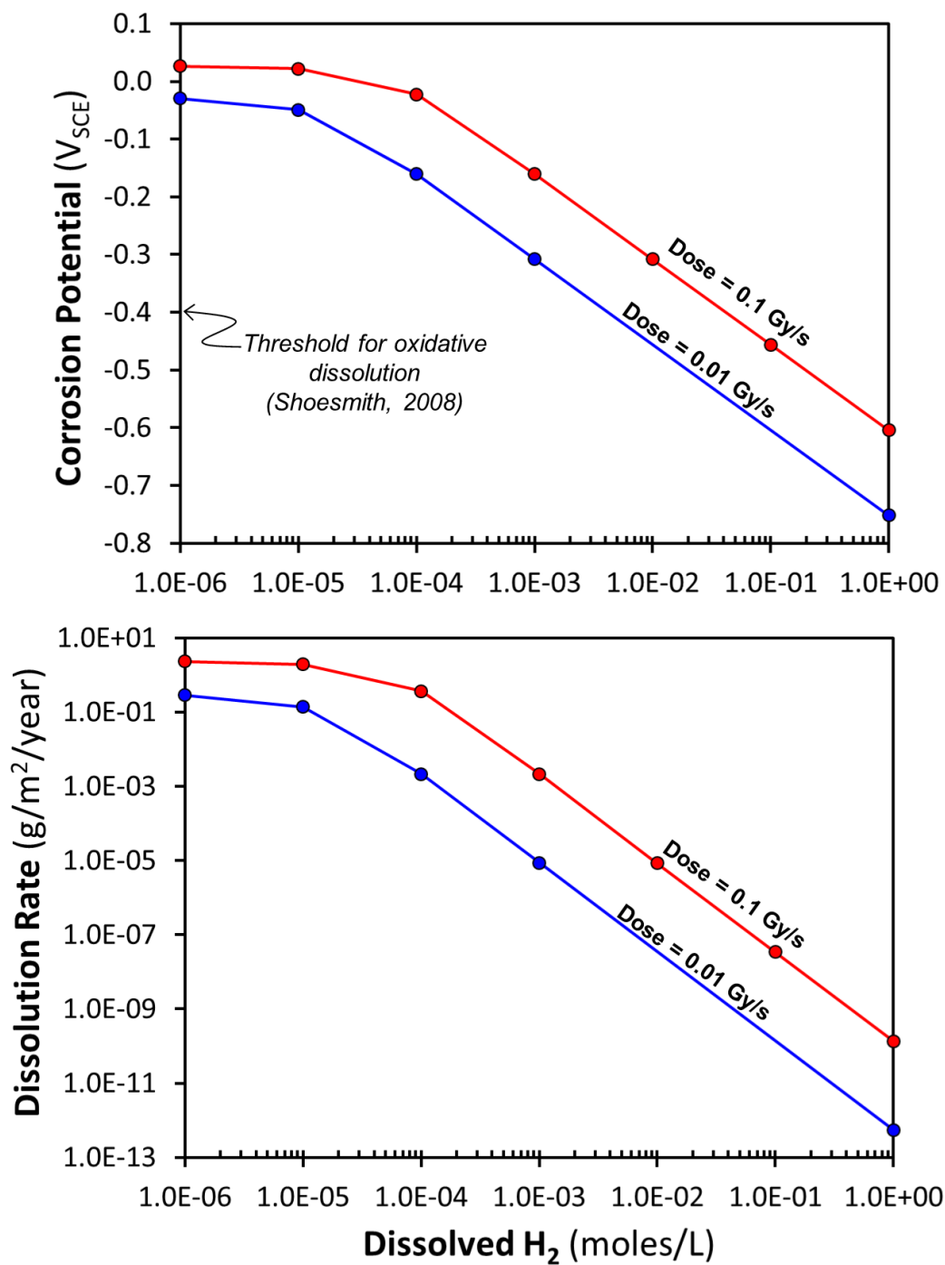
Figure 7.7. Fuel corrosion potential and dissolution rate as function of hydrogen concentration for two typical dose rates. Surface coverage of NMP is set at 1%, for other assumptions see Table 7.1 above.
