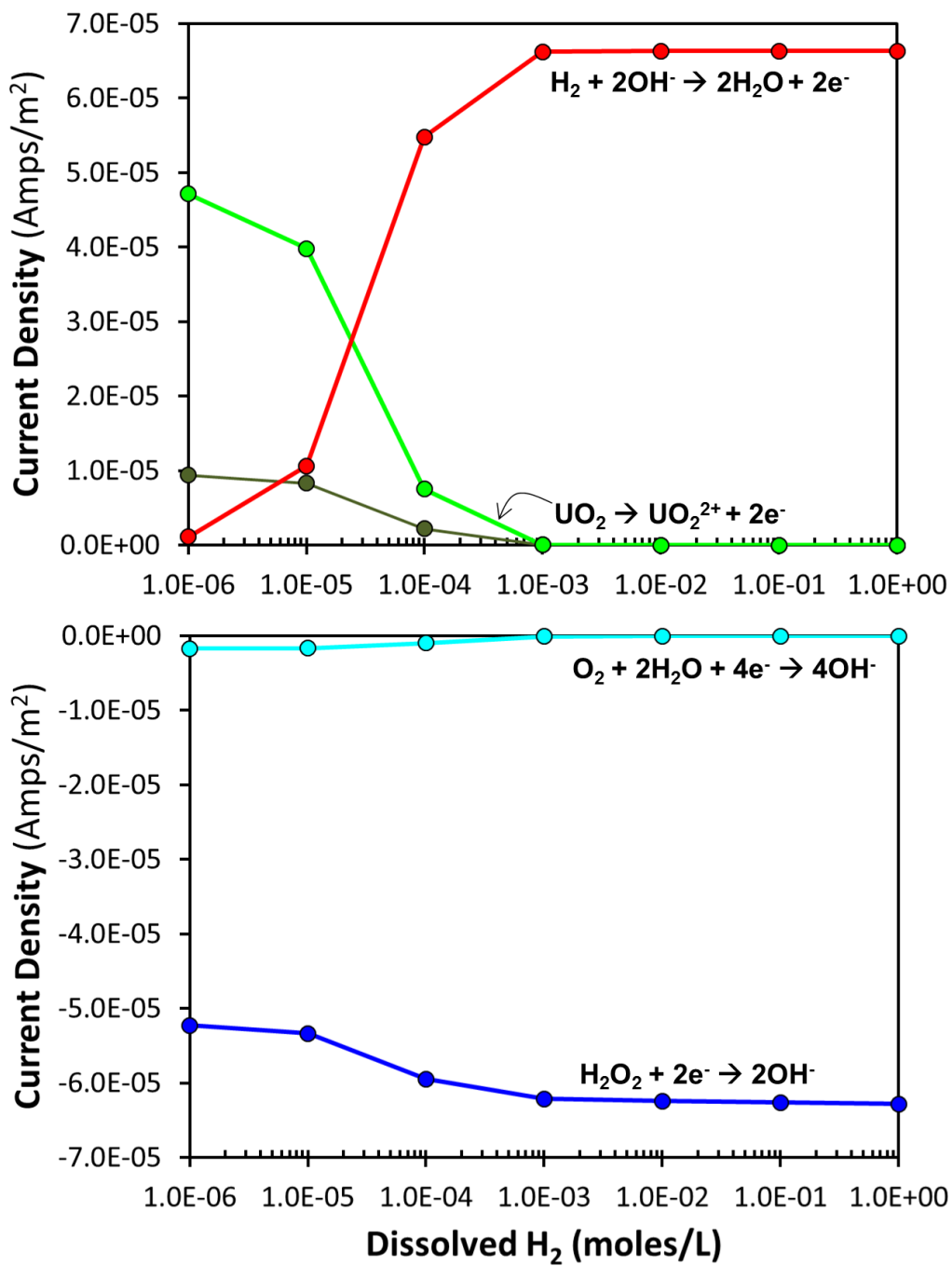
Figure 7.6. Current densities for the key reactions over a range of hydrogen concentrations. The anodic reactions are shown on the top plot, the cathodic reactions are shown on the bottom plot.
