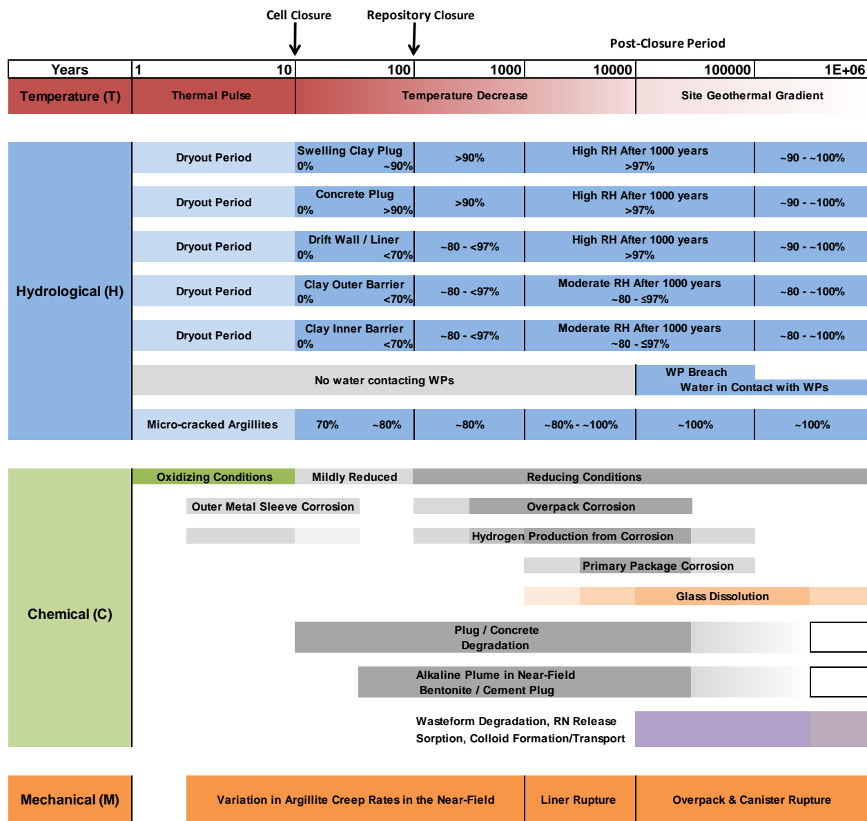
Figure 1.6. Schematic example of an idealized chronological evolution of the thermal, hydrologic, mechanical, and chemical (THMC) conditions for a generic argillite (clay/shale) disposal environment. Percentages in the hydrological part of the diagram represent percent of water saturation in the media.
