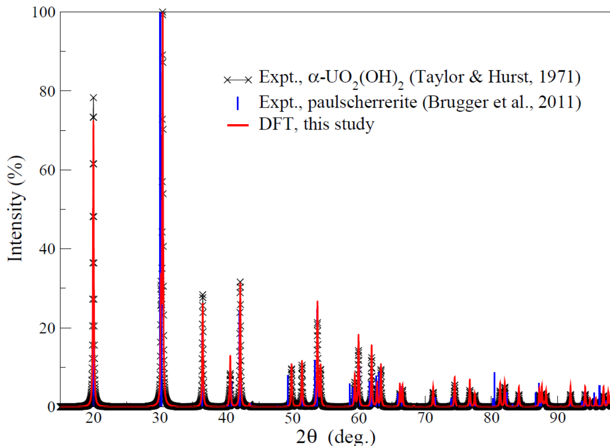
Figure 11.13. X-ray diffraction pattern of \alpha\text{-UO}_2(\text{OH})_2 . The experimental powder diffraction pattern for \text{Cu K}\alpha_1 radiation (Taylor and Hurst, 1971) is represented by a black line. The diffraction pattern simulated from the structure relaxed with DFT/PBE reported in the present study is shown in red. A full-width at half-maximum (FWHM) parameter of 0.2 2\theta was used in the simulation. The XRD pattern recorded for paulscherrerite, the mineral form of dehydrated schoepite (Brugger et al., 2011), is also reported for the sake of comparison.
