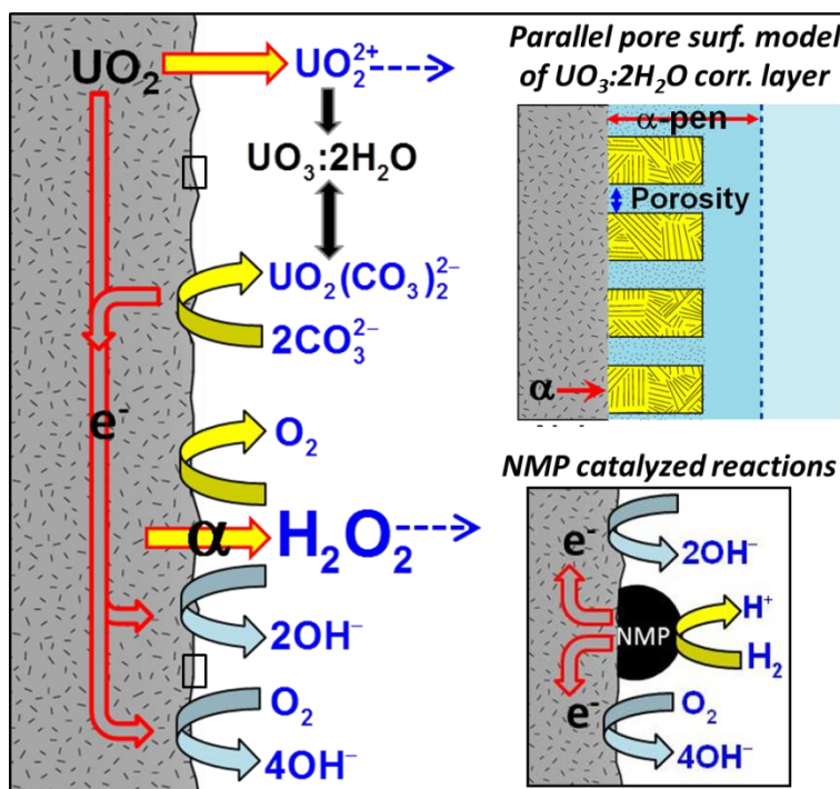
Figure 7.2. Key processes accounted for in the MPM. The corrosion layer is modeled as a set of parallel pores with fixed porosity and tortuosity. The noble metal particles (NMP) are modeled as reactive separate surface domain with its own set of surface reactions.
