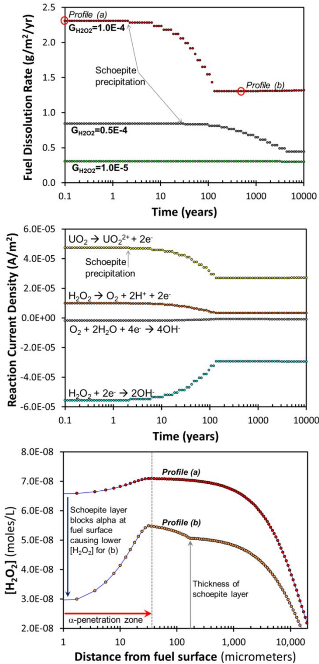
Figure 3.2. Results from recent MPM runs investigating the sensitivity of fuel degradation rate to changes in the G-value for H 2 O 2 in mole/(J/kg)/second (top). Individual time steps are represented as single data points. The middle diagram shows the reaction current densities (G H 2 O 2 =1.0E-5) for the redox reactions that determine the fuel corrosion potential and fuel degradation rate. The bottom diagram shows H 2 O 2 concentration profiles for the two time steps identified in the top diagram.
