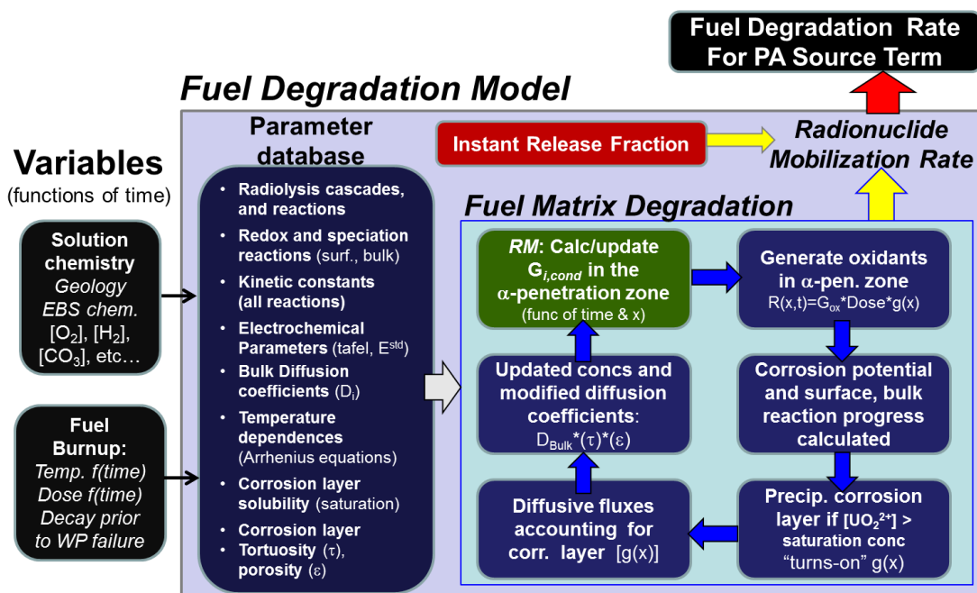
Figure 4.1. Summary information flow diagram highlighting the coupling of radiolysis, matrix, and instant release process modules within the FDM (MPM shown by blue boxes, RM by green box, and IRF by red box), and PA.
