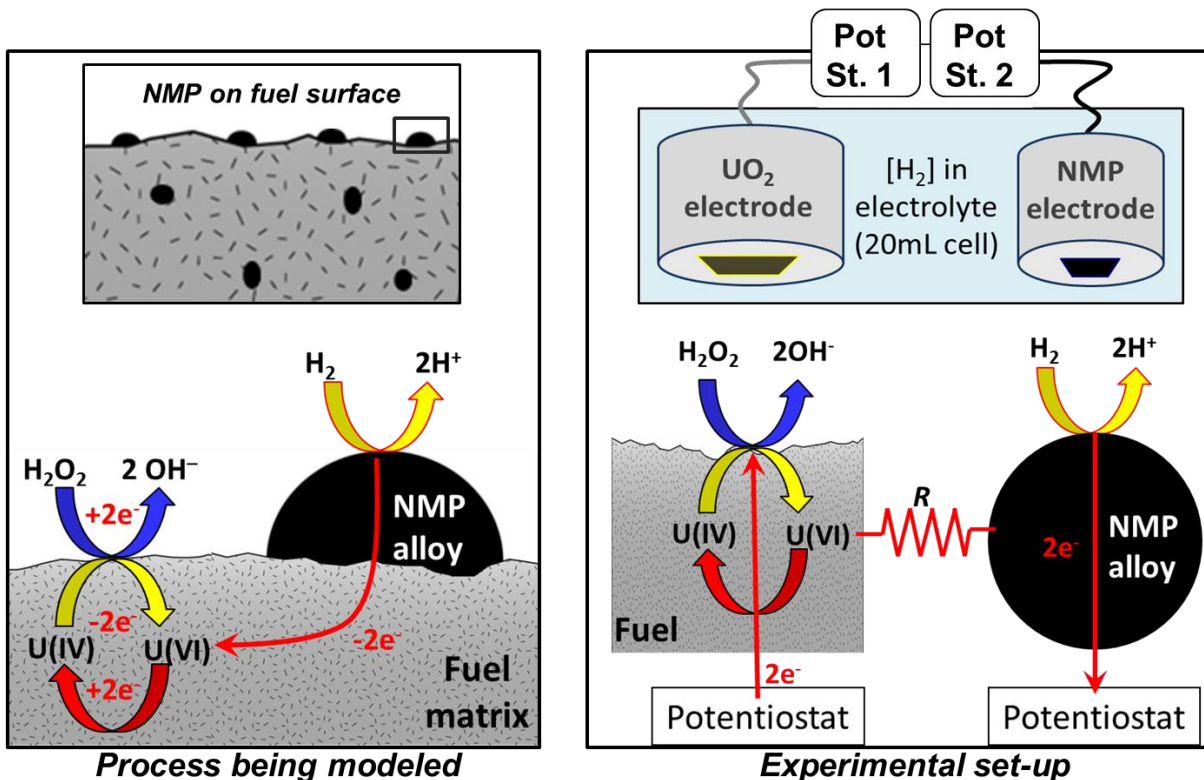
Figure 7.3. Schematic diagram showing flow of electrons for surface catalyzed oxidation of hydrogen. The diagrams on left shows the processes being implemented as part of the MPM. The diagrams on the right show a simplified conceptual view of the processes and set-up that was used to perform the electrochemical experiments (experimental results presented below).
