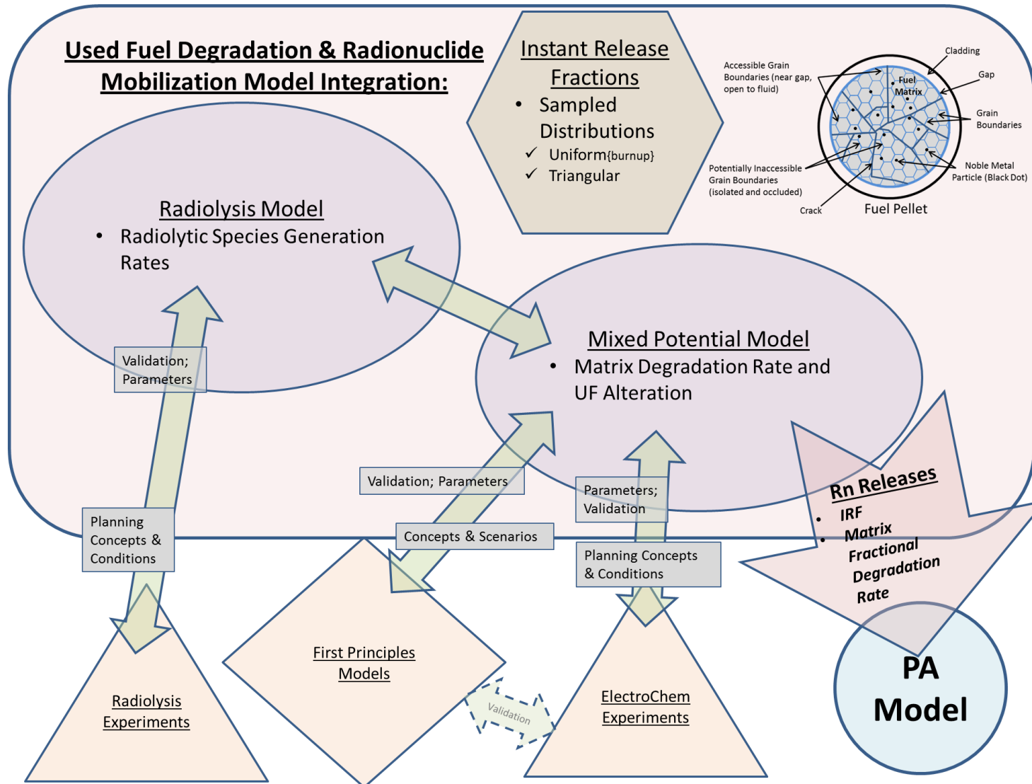
Figure ES-1. Schematic diagram of the integration among activities for used fuel degradation and the connection to a performance assessment model. Experimental work (triangles) and first principles models (diamond) shown as underpinning process models.
