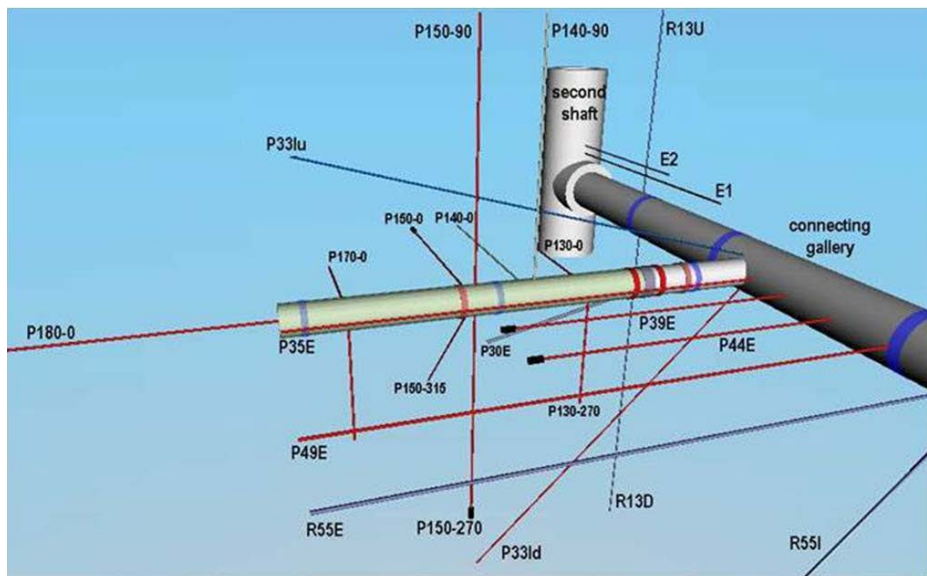
Figure 4.5-3 PRACLAY in situ experiment at HADES URL: Configuration of boreholes for pressure, stress, displacement, and water chemistry measurements (Li 2011).
