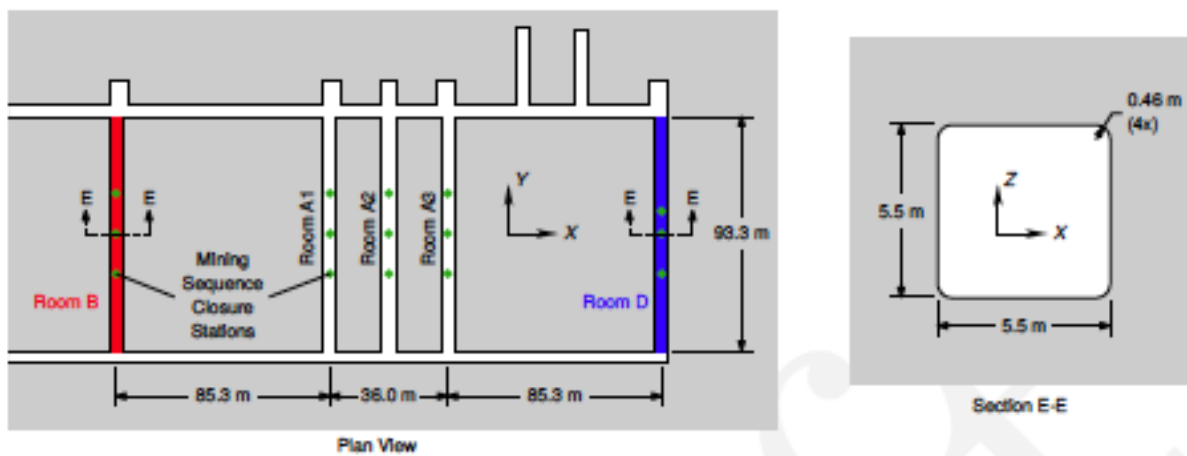
Figure 6.1-26 Rooms B and D dimensions (Reedlunn 2016).
