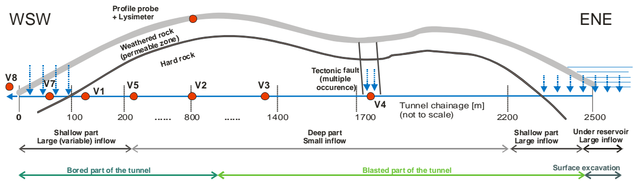
Figure 3.2-12 Profile of the tunnel with basic hydrogeological features and some measurement points (DECOVALEX web site, www.decovalex.org ).
