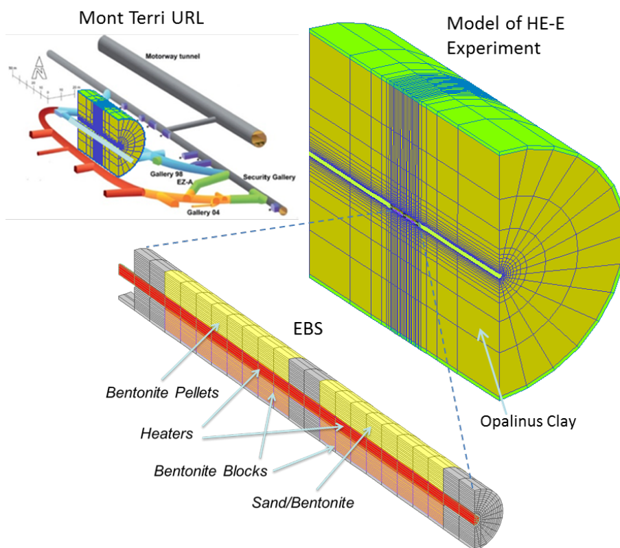
Figure 6.1-1 TOUGH-FLAC 3-D model of the Mont Terri HE-E experiment (Zheng et al. 2015).
