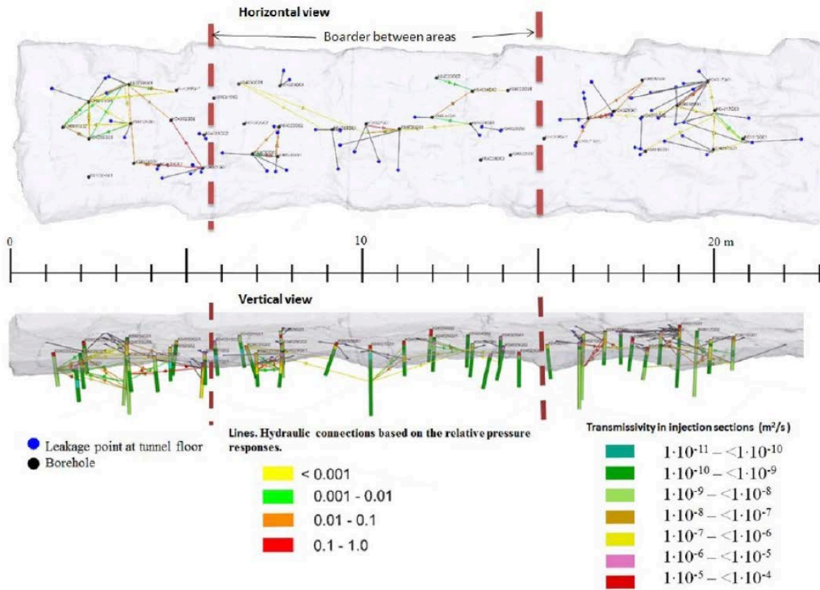
Figure 3.2-28 Top: hydraulic connectivity, expressed as relative pressure disturbance from <0.001 to 1. Bottom: transmissivities obtained from injection tests. The dotted red lines indicate areas where there is no observation of any hydraulic connectivity (Lanaro 2016).
