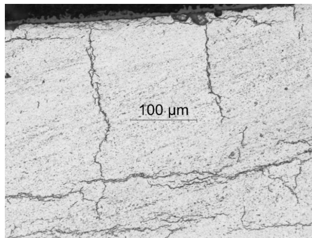
Figure 35: Longest radial hydride observed (at 200X) on the 646B6 surface.
