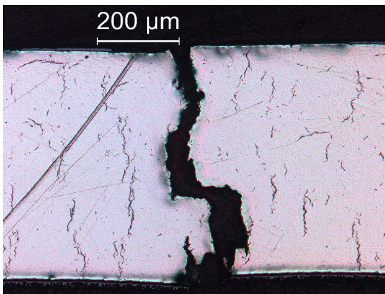
Figure 11: Through-wall crack in HBU-fuel M5 ® ring tested at 23°C following 350°C/89-MPa RHT.
