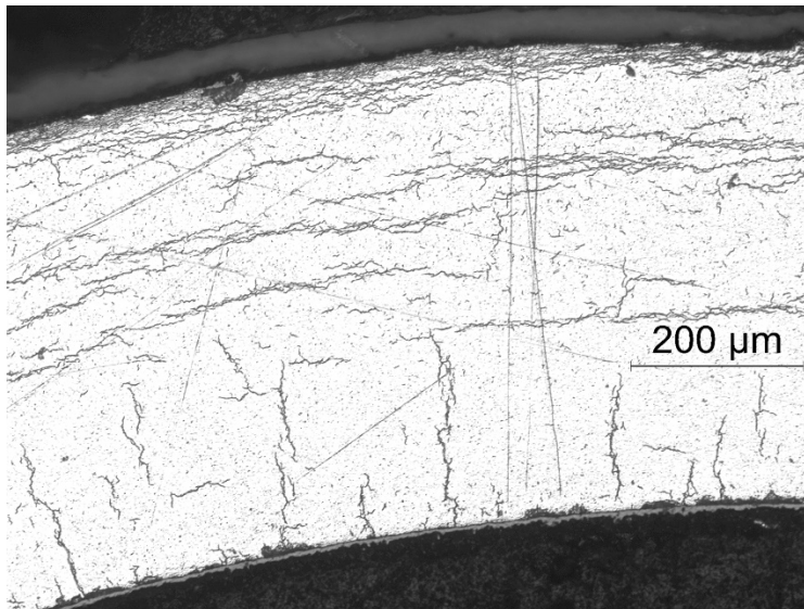
Figure 46: Maximum RHCF (44%) observed at 100X on the 8A surface.
