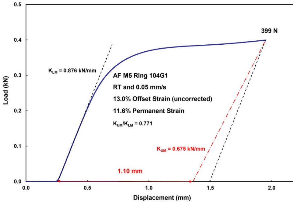
Figure 21: Load-displacement curve for AF 17×17 M5 ® ring displaced to 1.7 mm at RT and 0.05 mm/s.
