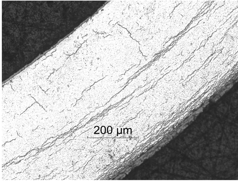
Figure 37: Maximum RHCF (33%) for surface 3A, which was 11 mm from the bottom insert.
