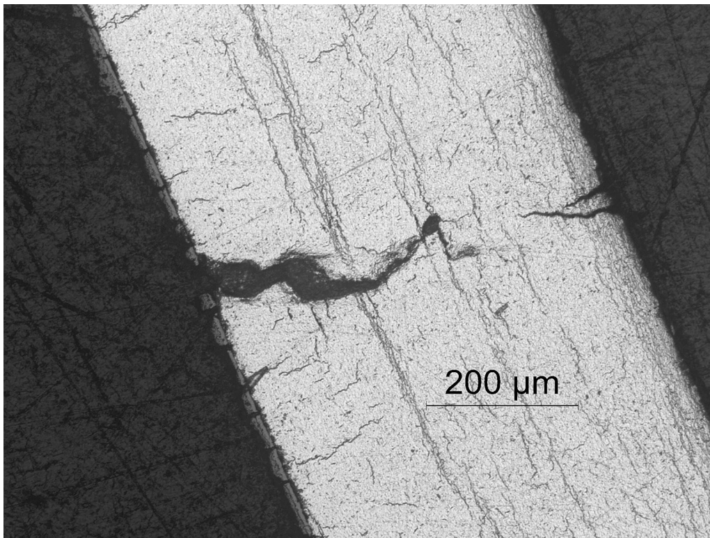
Figure 43: Cracking observed at the assumed 12 o'clock location of the bottom end of Ring 4.
