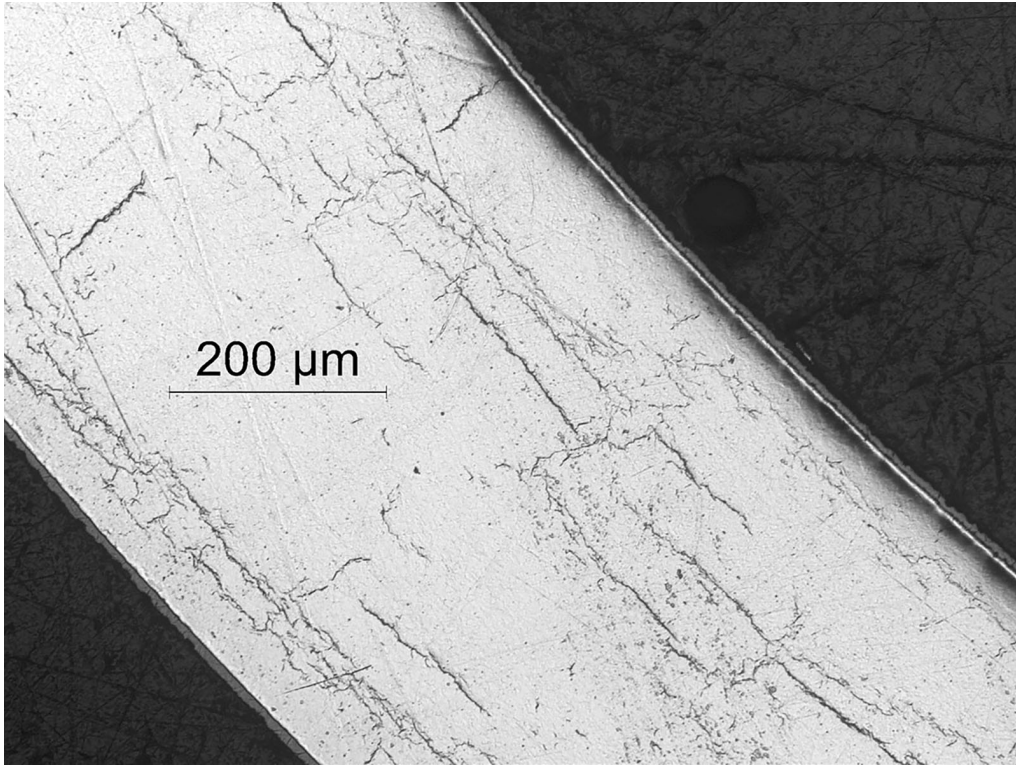
Figure 65: 100X image of a thicker radial hydride (20% RHCF) observed at the 7 o'clock location of the M5 ® surface 654B6 located at \approx 3360 mm from the bottom of FHT fuel rod 30AE14.
