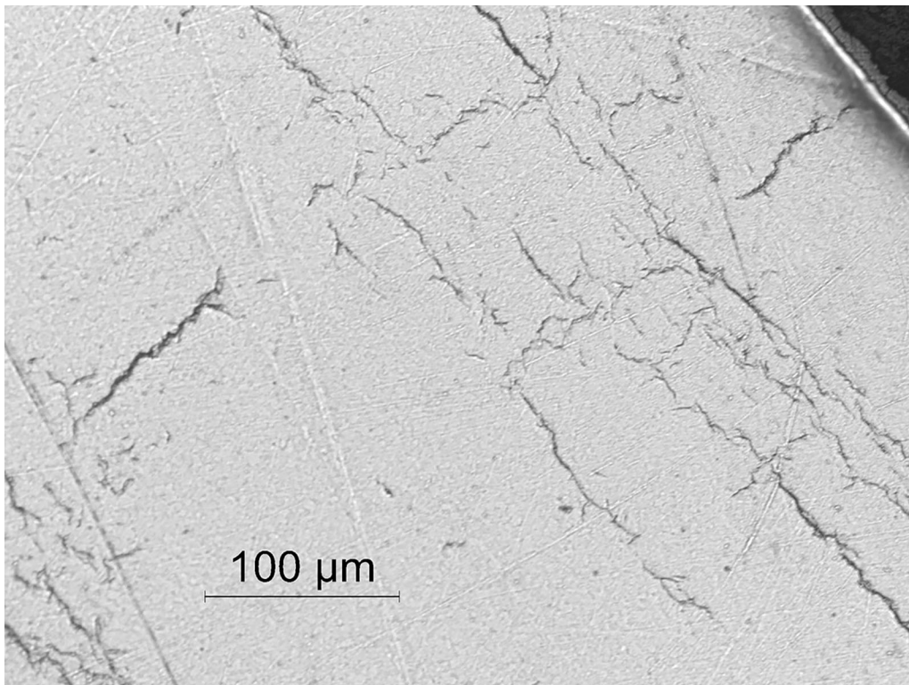
Figure 66: 200X image of a thicker radial hydride (20% RHCF) observed at the 7 o'clock location of the M5 ® surface 654B6 located at \approx 3360 mm from the bottom of FHT fuel rod 30AE14.
