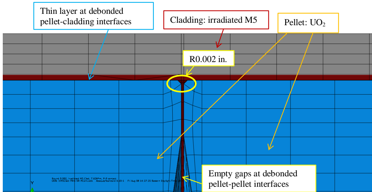
Fig. 57. Enlarged area in Fig. 45 for the cases of empty gaps at debonded pellet-pellet interfaces, and a thin layer filled at the debonded pellet-clad interfaces.
