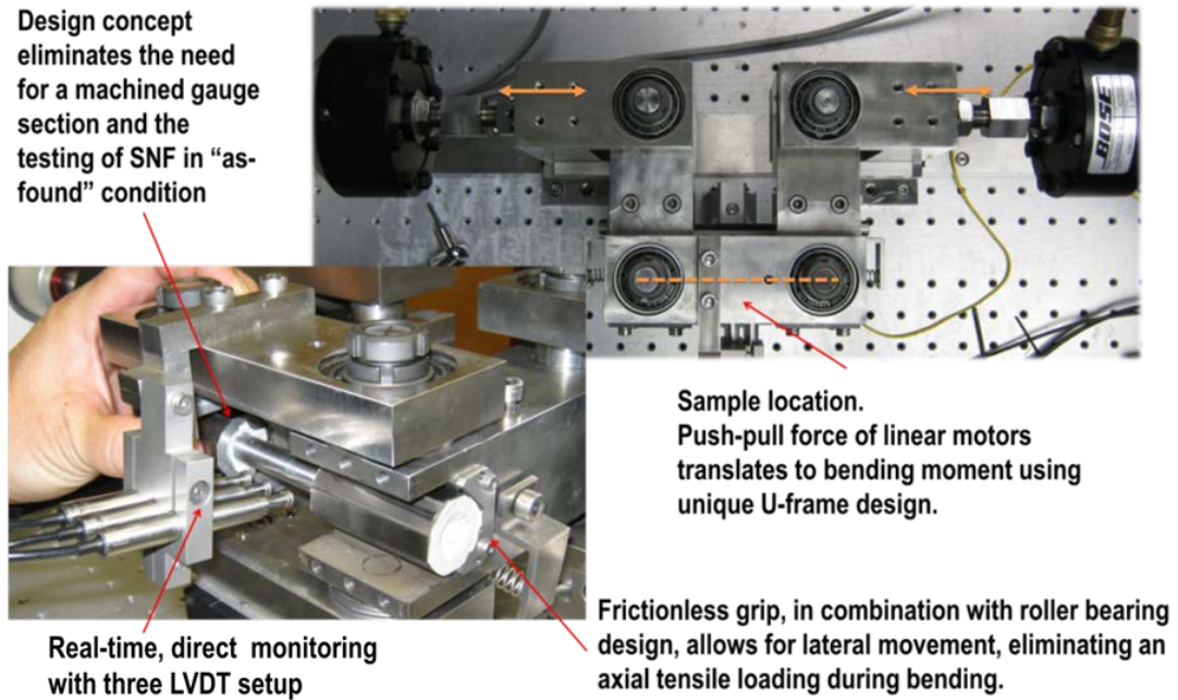
Fig. 63. CIRFT testing system with horizontal U-frame test setup integrated to Bose dual LM2 TB.
