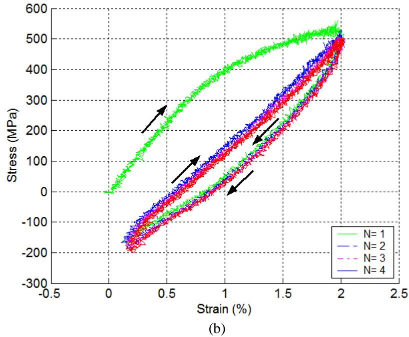
Fig. 17. (a) Moment-curvature curves and (b) equivalent stress-strain curves based on the first four loading cycles for specimen NA3 (651D3).
