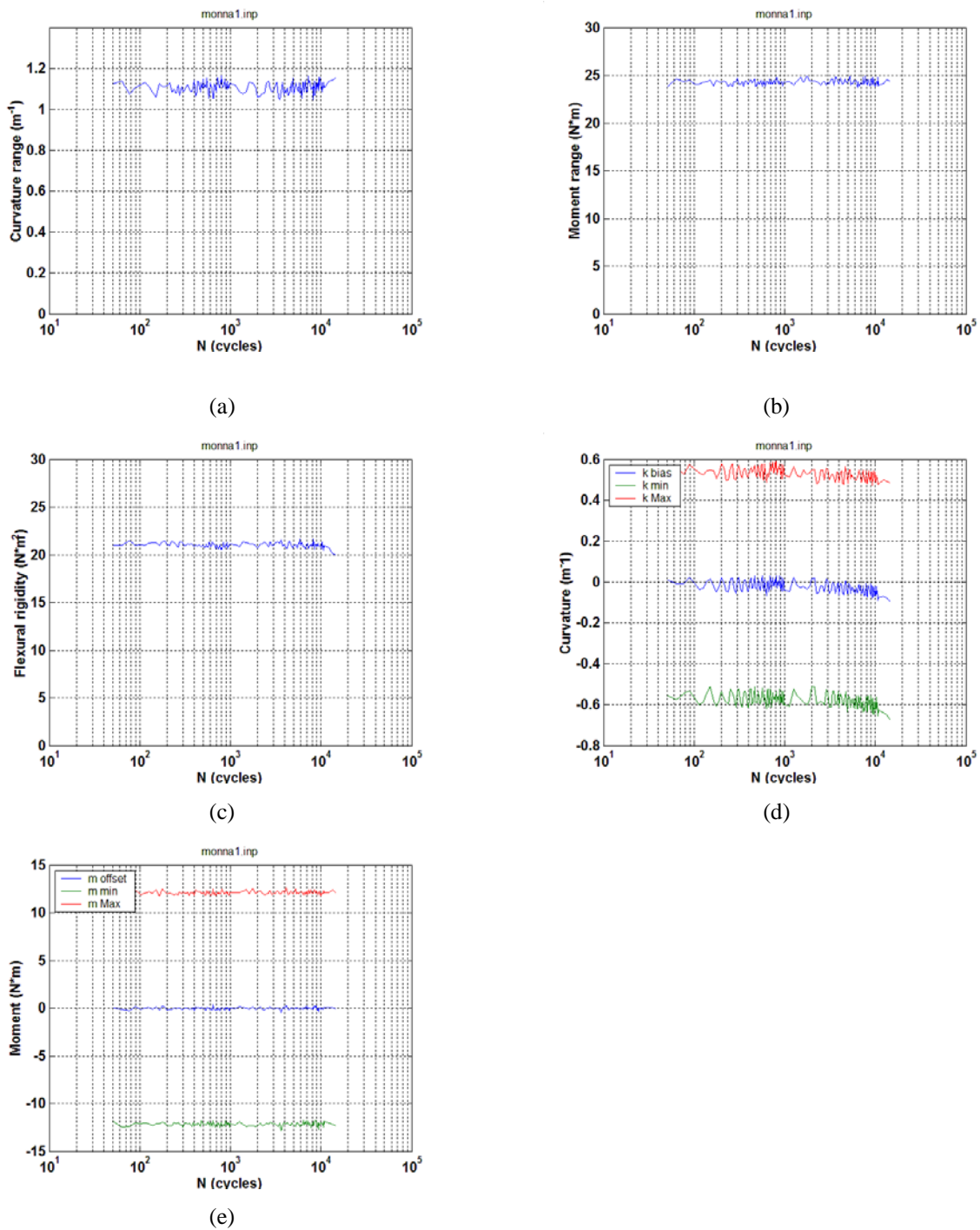
Fig. 25. Variations of (a) curvature range, (b) applied moment range, (c) flexural rigidity, (d) maximum and minimum values of curvature, and (e) maximum and minimum values of moment as a function of number of cycles for NA1 (651B2); N_f = 1.57 \times 10^4 cycles under \pm 12.70 N·m, 5 Hz.
