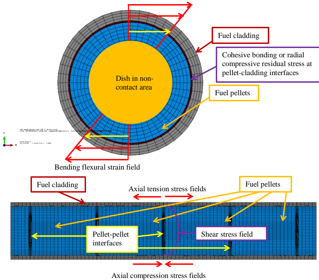
Fig. 50. Transportation-induced reversal bending stress fields in a UNF system.
