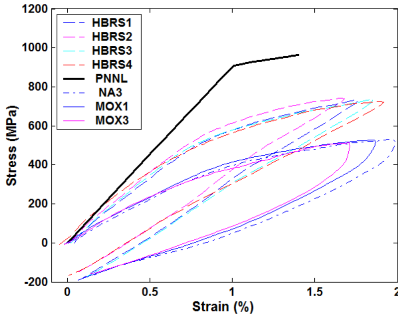
Fig. 38. Stress-strain curves based on static testing results for HBR, NA and MOX UNF. Relative displacement was 24.00 mm; the loading/unloading rate at each point was 0.1/0.2 mm/s.
