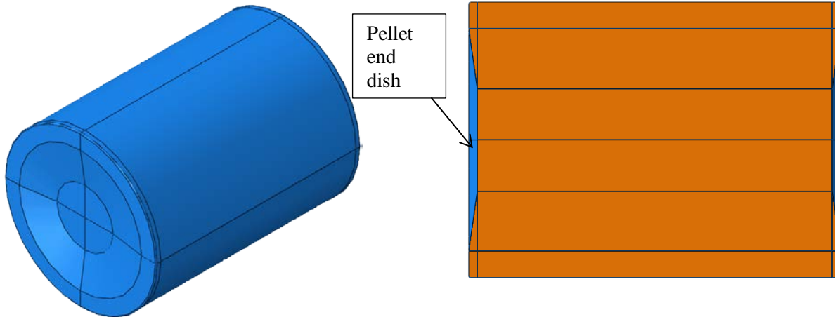
Fig. 44. FEA model of fuel pellet.
