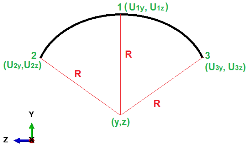
Fig. 64. Sketch for curvature calculation.
