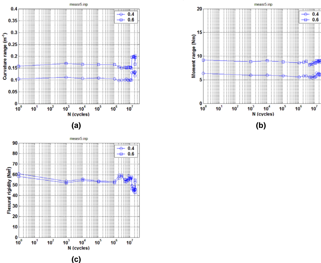
Fig. 12. Variations of (a) curvature range, (b) applied moment range, and (c) flexural rigidity as a function of number of cycles for R5 (606B3C); N = 2.23 \times 10^7 cycles under \pm 7.62 \text{ N}\cdot\text{m} 5 Hz.
