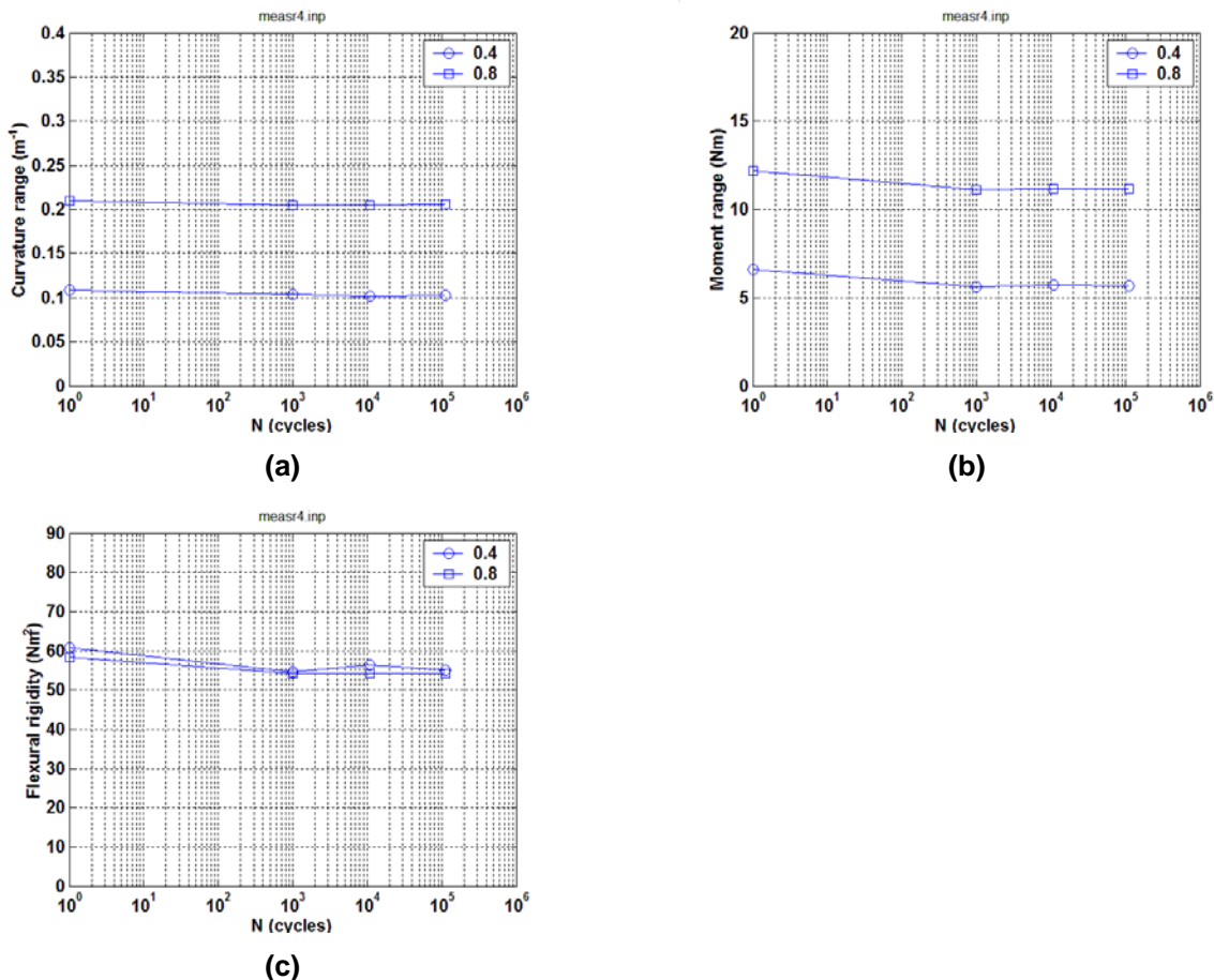
Fig. 10. Variations of (a) curvature range, (b) applied moment range, and (c) flexural rigidity as a function of number of cycles for R4 (606B3D); N_t = 2.7 \times 10^5 cycles under \pm 8.89 N·m 5 Hz.
