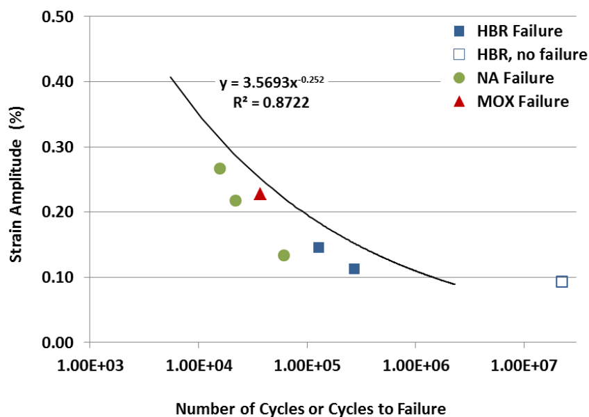
Fig. 40. Strain amplitudes as a function of number of cycles; results are based on CIRFT testing at 5 Hz. The power function was obtained from curve fitting based on the HBR data set [11].
