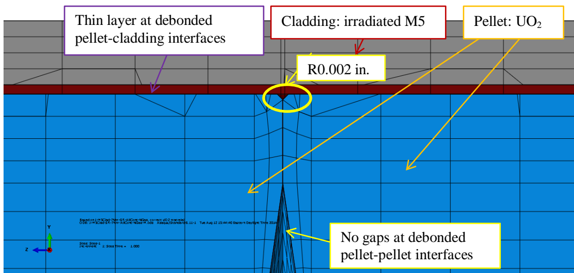
Fig. 60. Enlarged area in Fig. 45 for the case with no gaps at debonded pellet-pellet interfaces and a thin layer at debonded pellet-clad interfaces.
