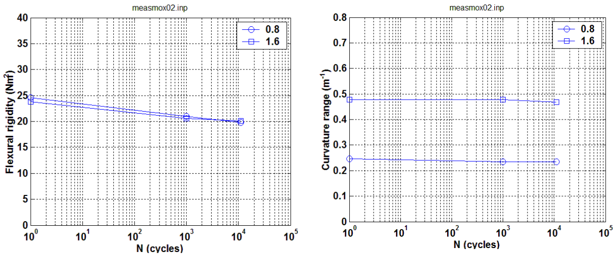
Fig. 49. ORNL hot cell CIRFT MOX2 data, flexural rigidity, and curvature.
