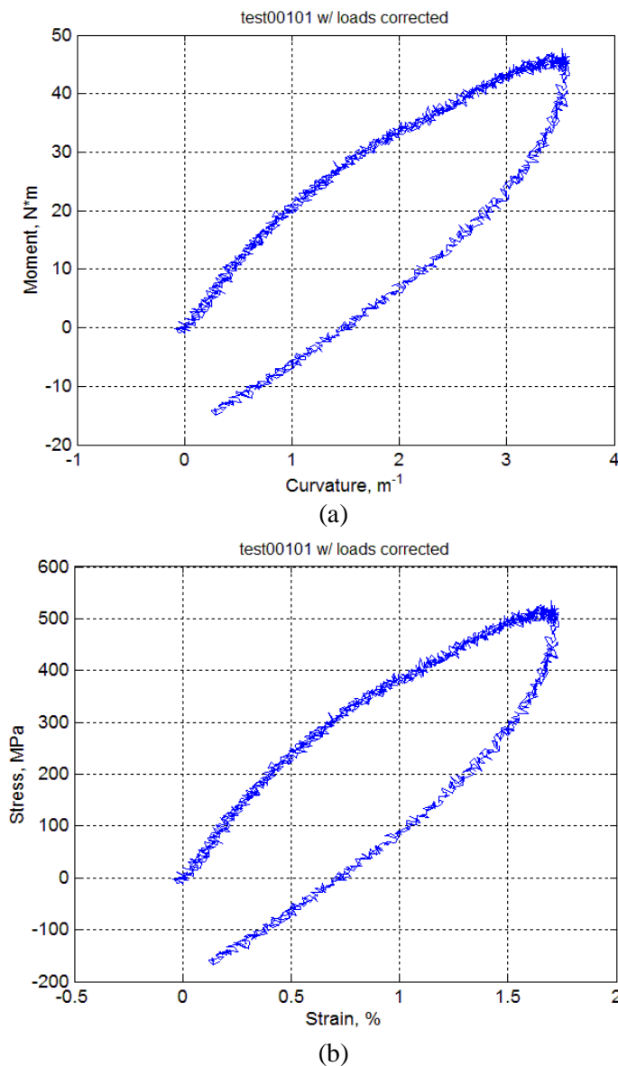
Fig. 21. (a) Moment-curvature curves and (b) equivalent stress-strain curves based on the first four loading cycles for MOX3 (MOX-A-13).
