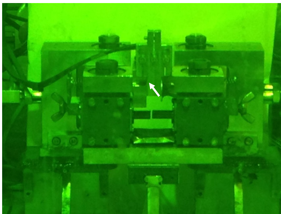
Fig. 30. Fracture location of NA2 (651C5), N_f = 2.2 \times 10^4 cycles under \pm 10.16 N·m, 5 Hz.
