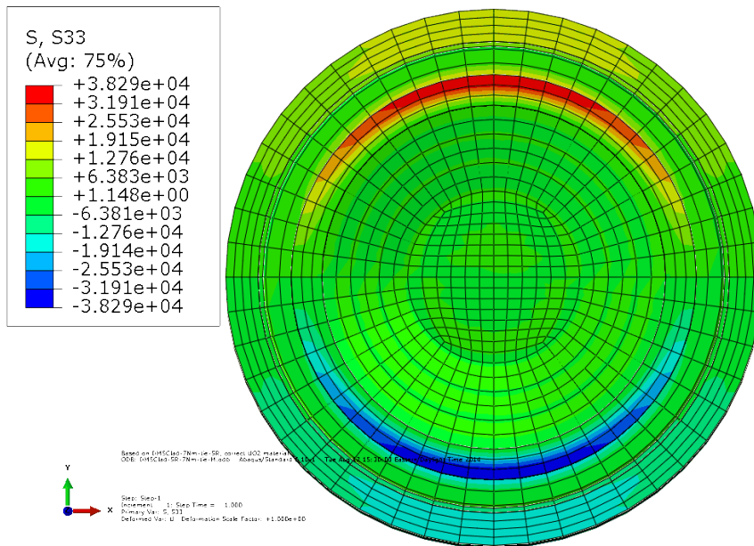
Fig. 47. Normal stress distribution and curvature results for clad-epoxy-pellet section model of M5 clad and six UO 2 pellets with perfect bonding.
