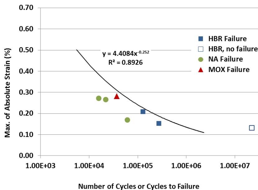
Fig. 41. Maxima of absolute strain extremes as a function of number of cycles; results are based on CIRFT testing at 5 Hz. The power function was obtained from curve fitting based on the HBR data set [11].
