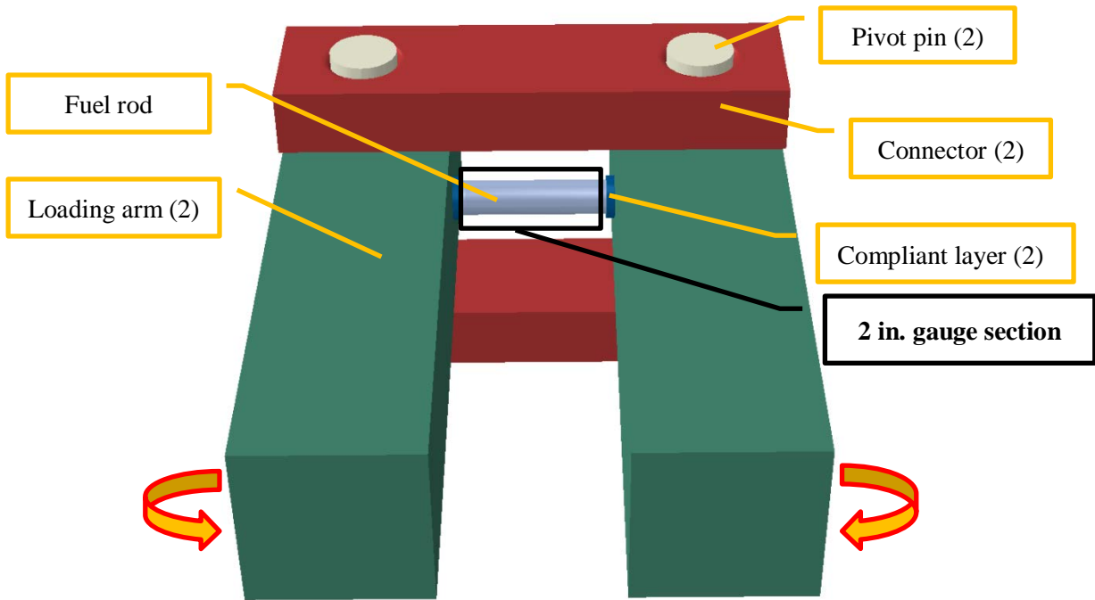
Fig. 42. Geometry of horizontal U-frame bending fatigue testing system with a coplanar rod configuration.
