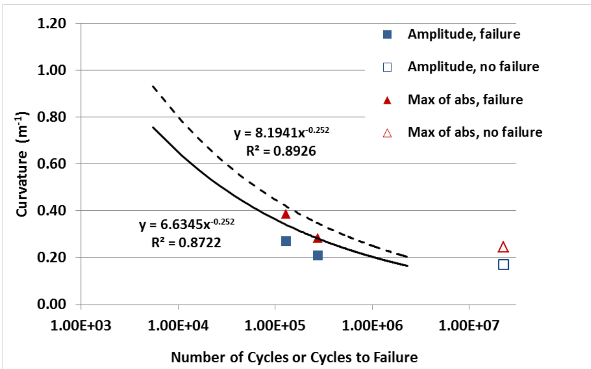
Fig. 13. Maxima of absolute (abs) curvature extremes and curvature amplitudes as a function of number of cycles. Solid markers represent tests with specimen failures; open markers indicate tests without failures. The power function was obtained from curve fitting based on the HBR data set [11]; solid line corresponds to amplitudes, and dash line corresponds to maxima of absolute.
