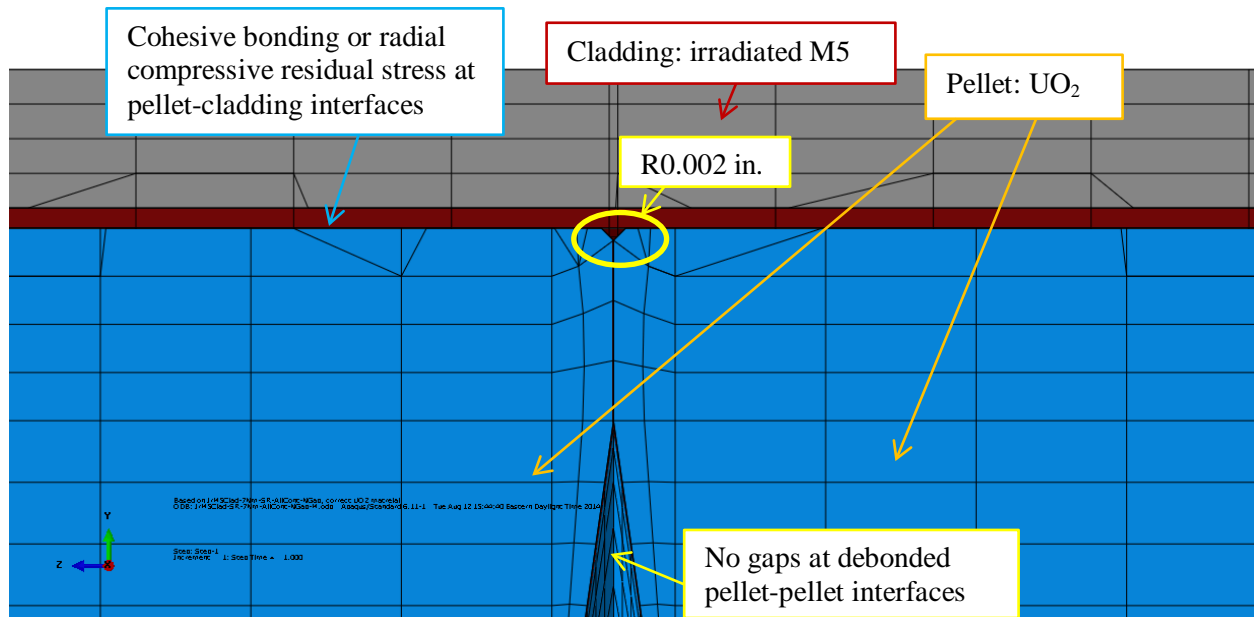
Fig. 54. Enlarged area in Fig. 45 for the case of no gaps at debonded pellet-pellet interfaces.
