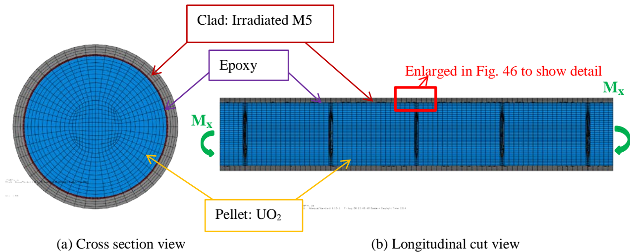
Fig. 45. Geometry of clad-epoxy-pellet two in. section model with six pellets and M5 Clad.
