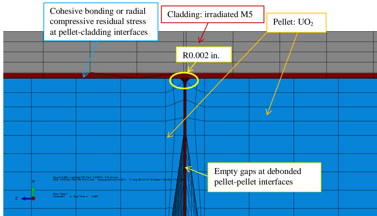
Fig. 51. Enlarged area in Fig. 45 for the case of empty gaps at debonded pellet-pellet interfaces.
