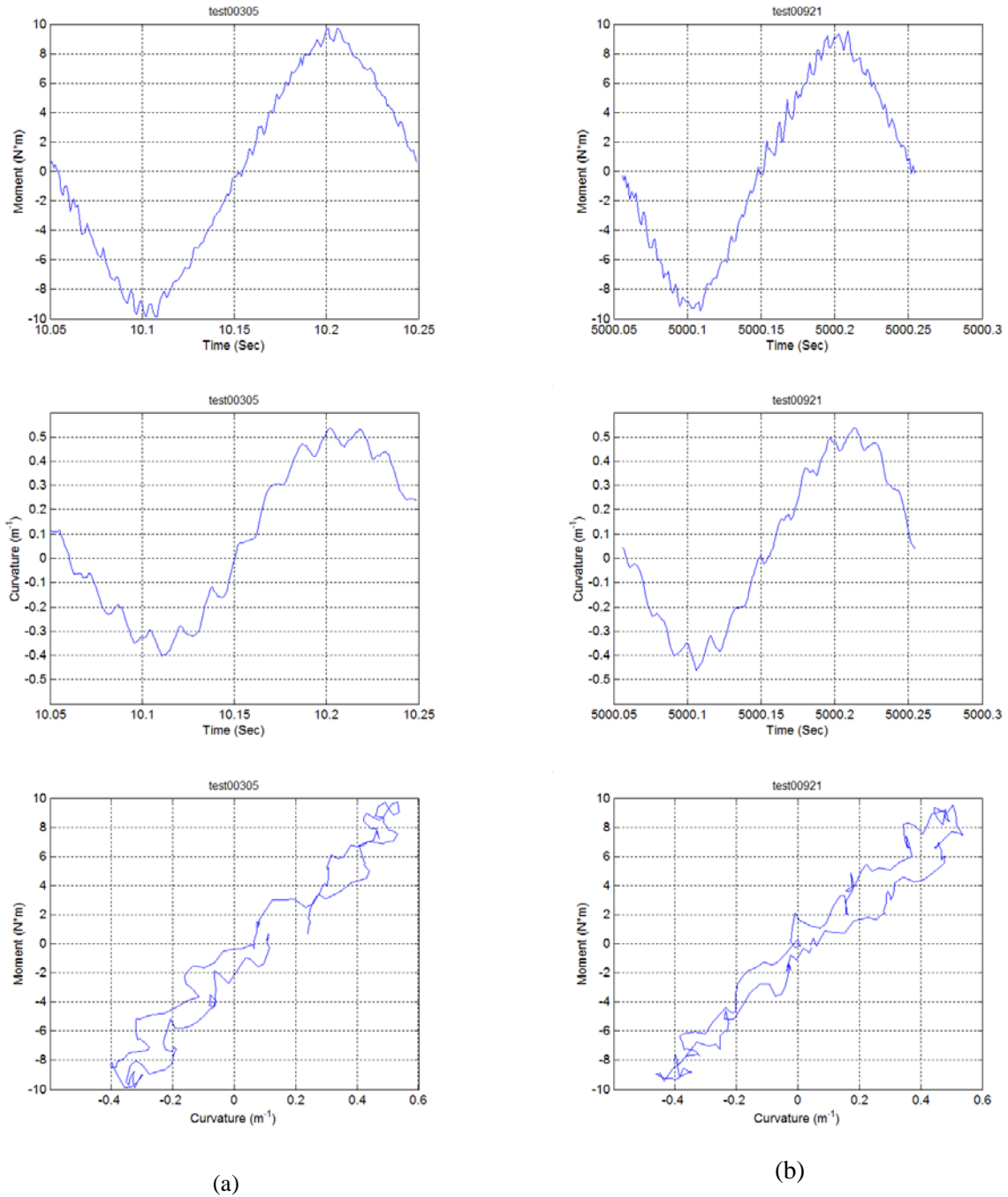
(a) (b) Fig. 37. Moment and curvature as a function of time and moment-curvature loops at (a) 50 and (b) 3.6 \times 10^4 cycles; results are based on on-line monitoring of MOX2 (MOX-A-12); N_f = 3.7 \times 10^4 cycles under \pm 10.16 N·m, 5 Hz.
