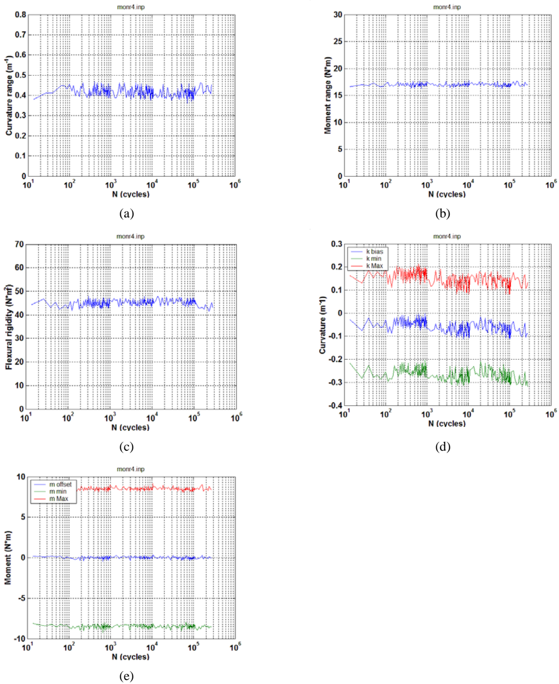
Fig. 9. Variations of (a) curvature range, (b) applied moment range, (c) flexural rigidity, (d) maximum and minimum values of curvature, and (e) maximum and minimum values of moment as a function of number of cycles for R4 (606B3D); N_f = 2.7 \times 10^5 cycles under \pm 8.89 N·m 5 Hz.
