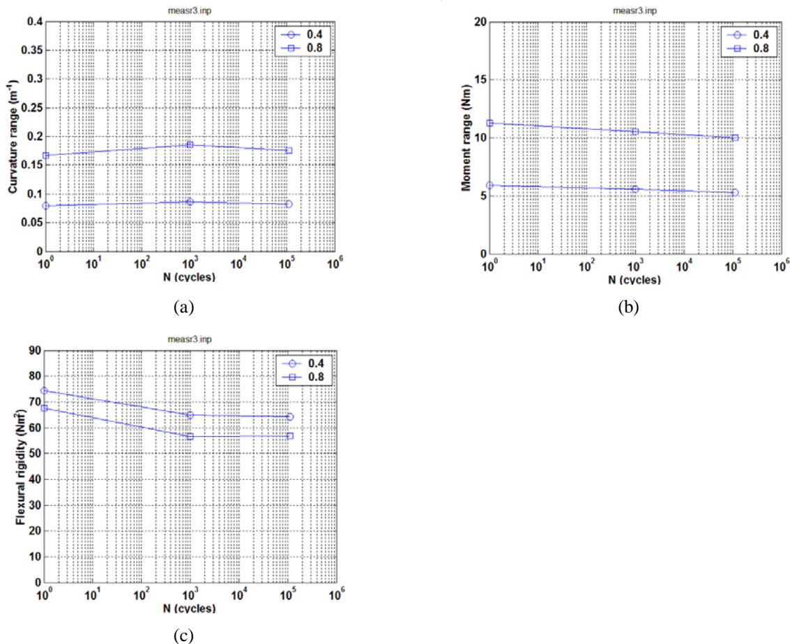
Fig. 8. Variations of (a) curvature range, (b) applied moment range, and (c) flexural rigidity as a function of number of cycles for D13/R3 (606B3E); N_f = 1.29 \times 10^5 cycles under \pm 13.72 \text{ N}\cdot\text{m} 5 Hz.
