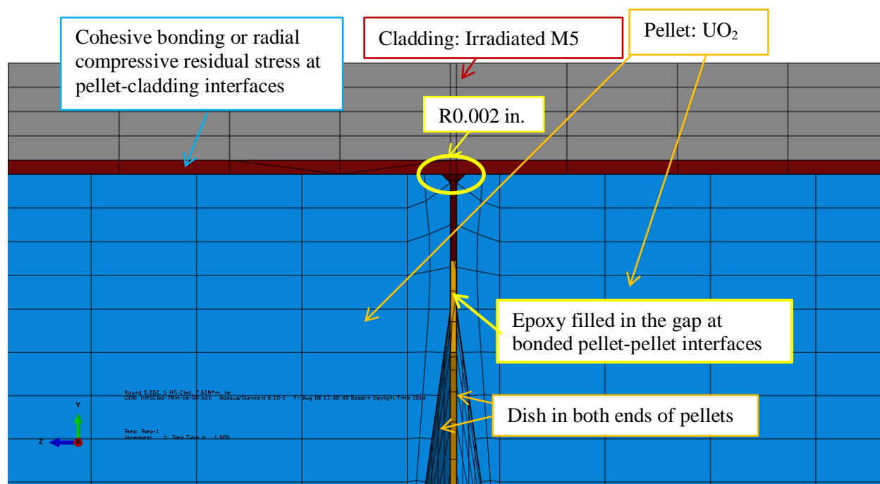
Fig. 46. Detail from Fig. 45 for the perfect bond case.
