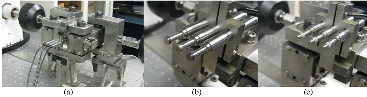
Fig. 4. (a) Three curvature LVDTs being held against the rod; (b) LVDT clamp open to show (b) flat probe and (c) chisel probe.
