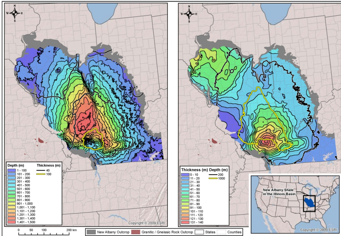
Figure 2-5. Depth and isopach maps of the New Albany Shale, Illinois Basin. Figure produced by LANL from shale data populated into the GIS database.
