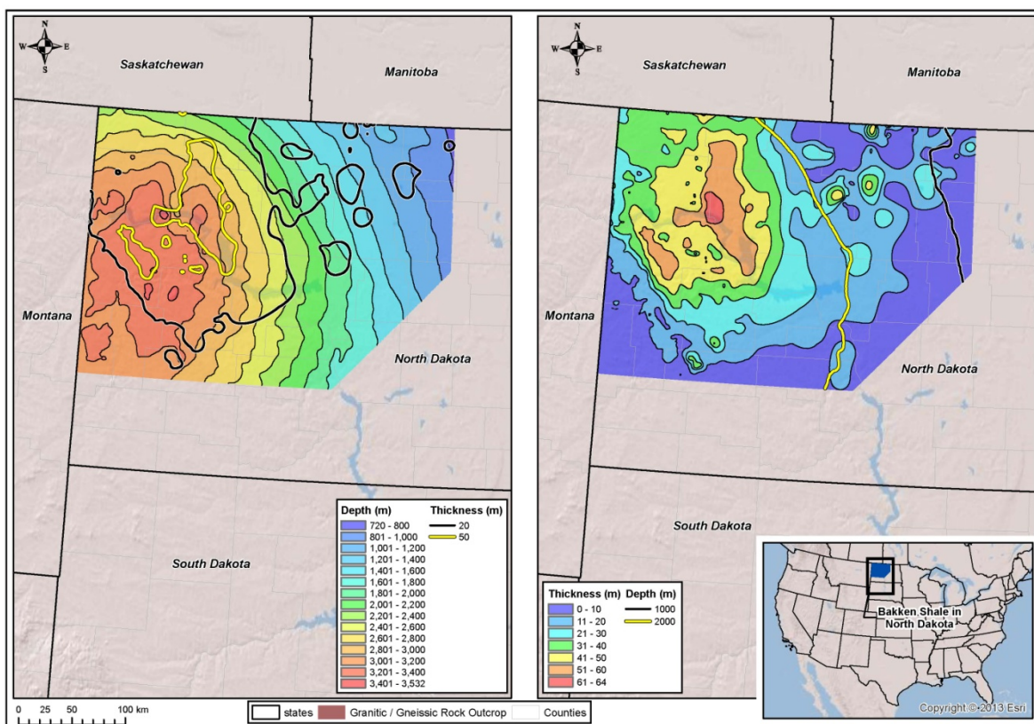
Figure 2-19. Depth and isopach maps of the Bakken Formation, Williston Basin. Figure produced by LANL from shale data populated into the GIS database.
