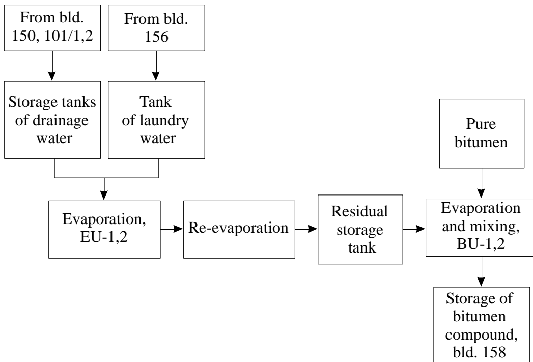
Figure D-2. The process of the collection of the liquid radioactive waste and the following bituminisation at INPP
