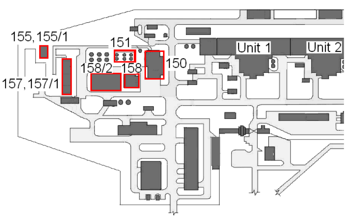
Figure D-1. Layout of radioactive waste facilities at INPP
