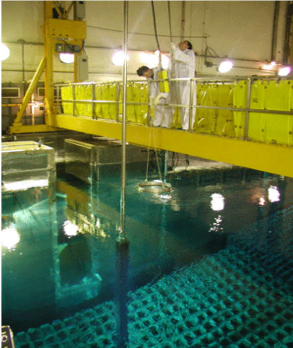
Figure 11: Krško NPP spent fuel pool
