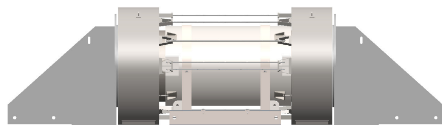
Cask in Transport Configuration (Side View)
