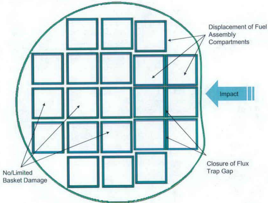
Figure 20. Radial Cross-Section Sketch of a Damaged PWR TAD Canister Depicting Basket Damage Considered Representative of a Horizontal Impact Event
