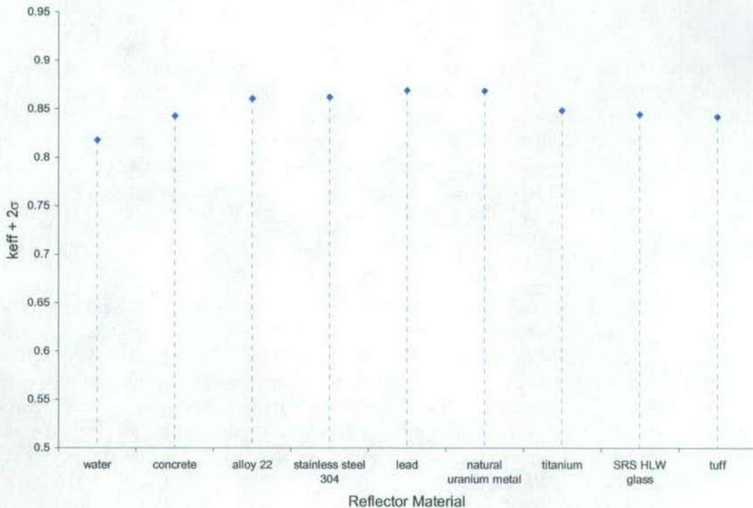
Figure 37. Variation of k_{eff} + 2\sigma with Close Fitting Full-Thickness (I.E. 30 cm) Reflector Material, for Single Damaged (Maximum Flux Trap Gap Collapse) and Partially Flooded (300 Liters Water Moderator) BWR TAD Canister Containing Intact, Damaged (Maximum Fuel Assembly Birdcaging), Representative CSNF
