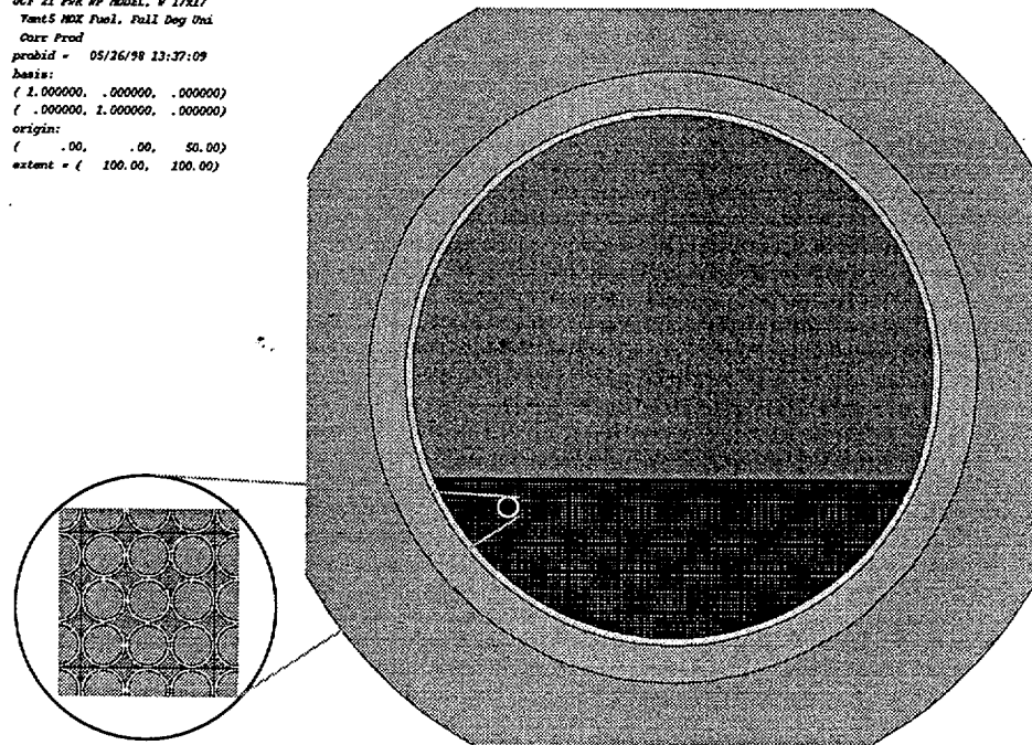
Figure 5.4-8. Degraded 21 PWR MOX WP with fuel rods collapsed to bottom of package surrounded by uniformly distributed basket corrosion products
