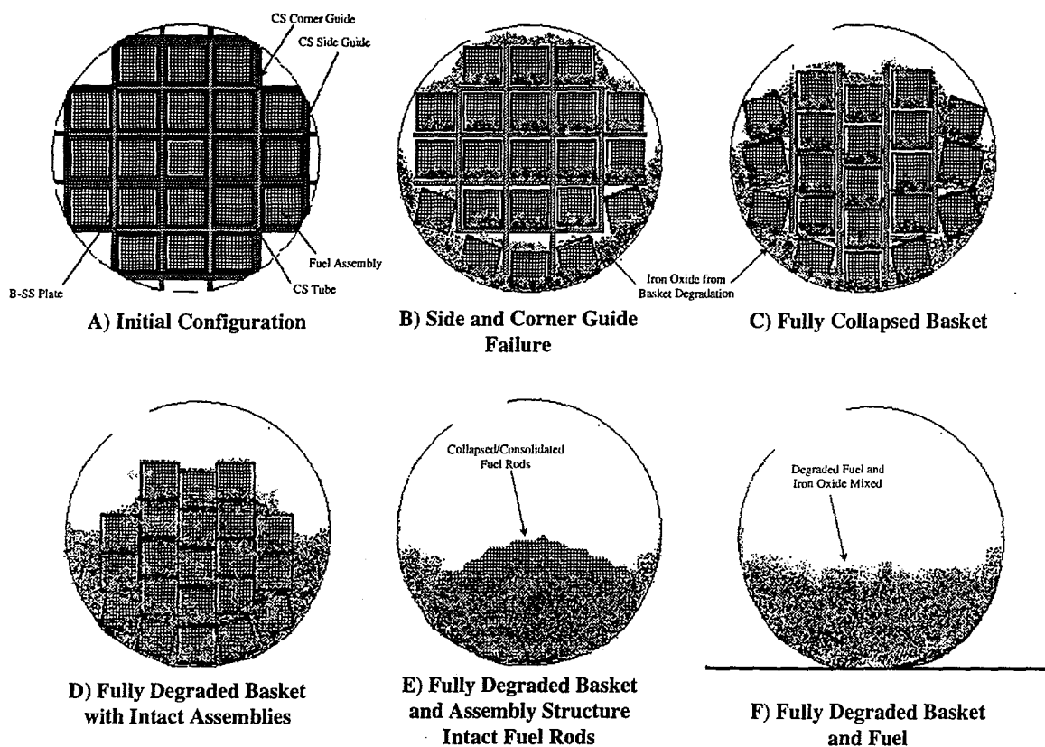
Figure 2-1. Degradation sequence of 21 PWR basket structure following WP breach
