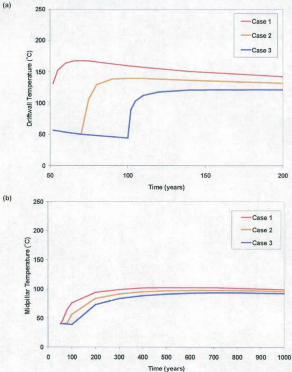
Figure 6-18. Postclosure Drift-Wall Temperature versus Time for Cases 1 through 3 for the Tptll Unit at the P2WR5C10 Location: (a) Drift-Wall Temperatures and (b) Mid-pillar Temperatures
