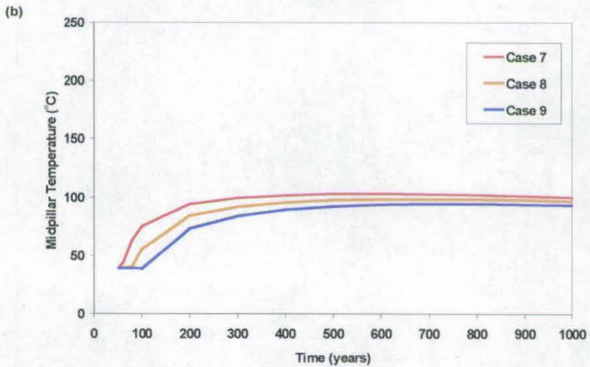
Figure 6-20. Postclosure Drift-Wall Temperatures versus Time for Cases 7 through 9 for the Tptpl Unit at the P2WR5C10 Location: (a) Drift-Wall Temperatures and (b) Mid-pillar Temperatures
