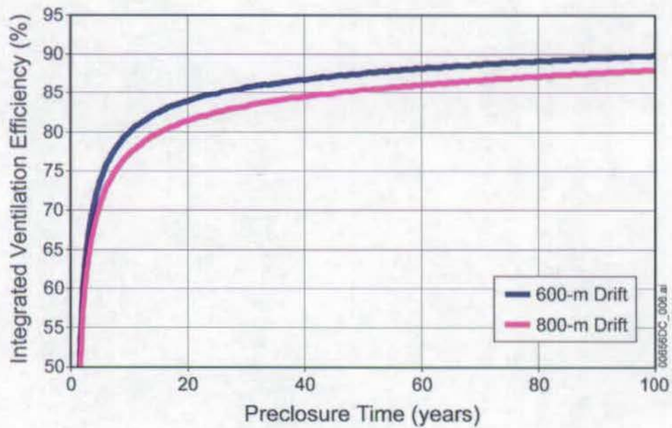
Figure 6-6. Integrated Ventilation Efficiency for Cases 1 through 3 in the Tptpl Unit
