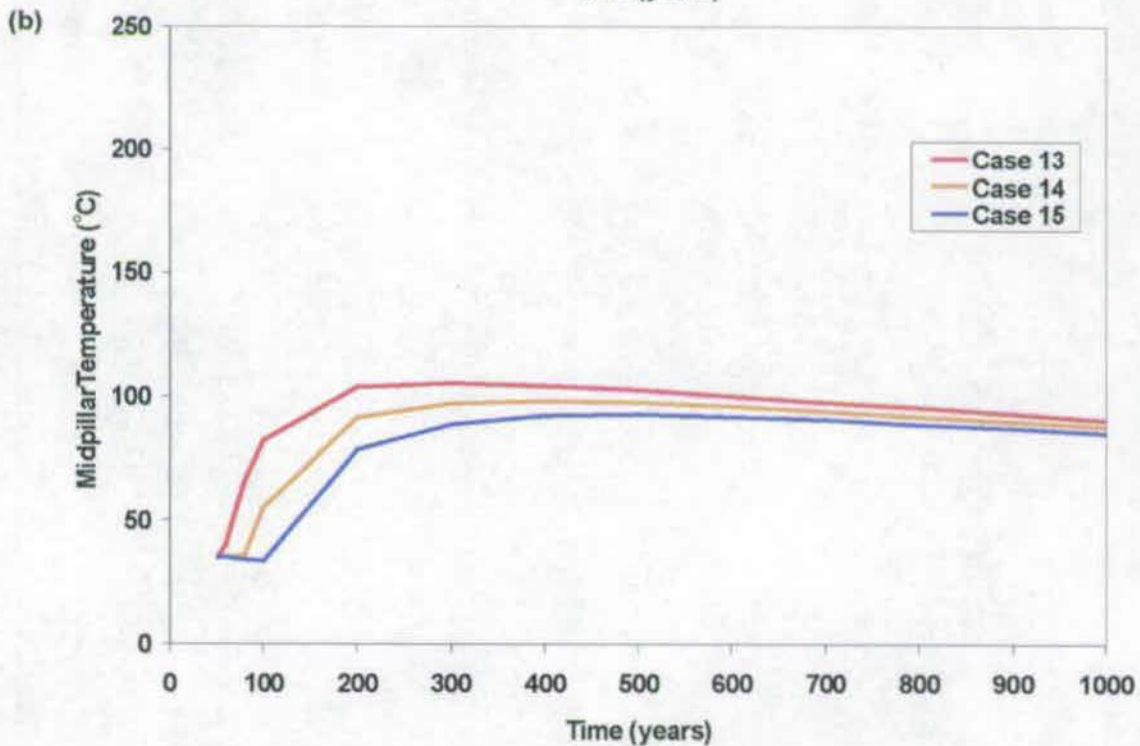
Figure 6-22. Postclosure Drift-Wall Temperatures versus Time for Cases 13 through 15 for the Ttpul Unit at the P2WR5C10 Location: (a) Drift-Wall Temperatures and (b) Mid-pillar Temperatures
