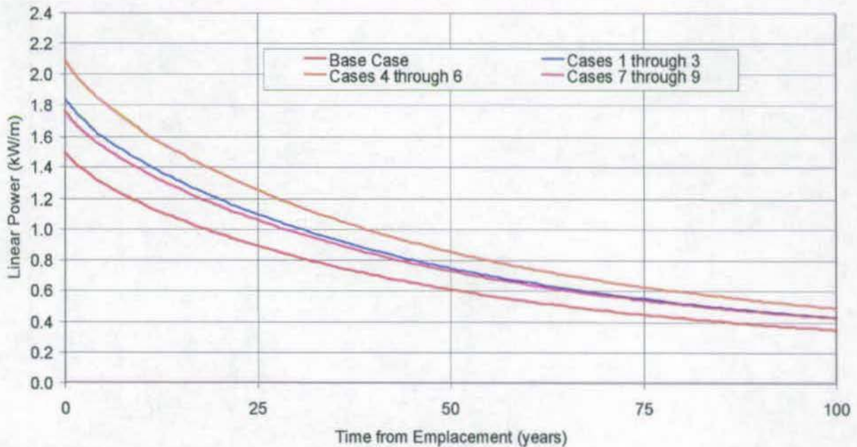
Figure 6-4. Replacement of the DHLW Packages with Hypothetical Packages Having Average Output
