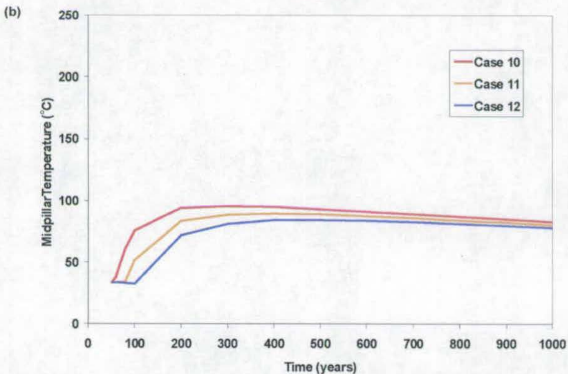
Figure 6-21. Postclosure Drift-Wall Temperatures versus Time for Cases 10 through 12 for the Tptpul Unit at the P2WR5C10 Location: (a) Drift-Wall Temperatures and (b) Mid-pillar Temperatures
