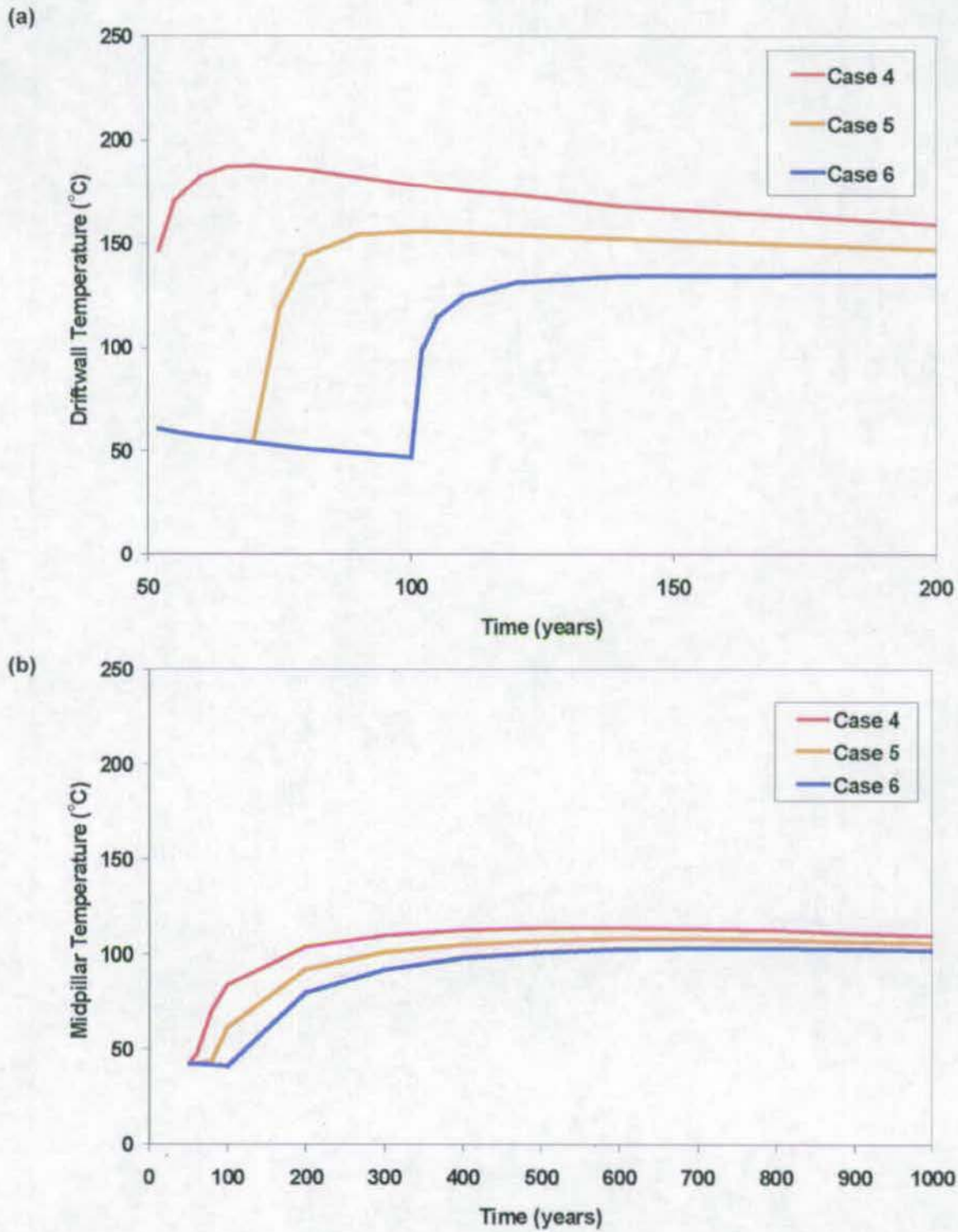
Figure 6-19. Postclosure Drift-Wall Temperature versus Time for Cases 4 through 6 for the Tptpl Unit at the P2WR5C10 Location: (a) Drift-Wall Temperatures and (b) Mid-pillar Temperatures
