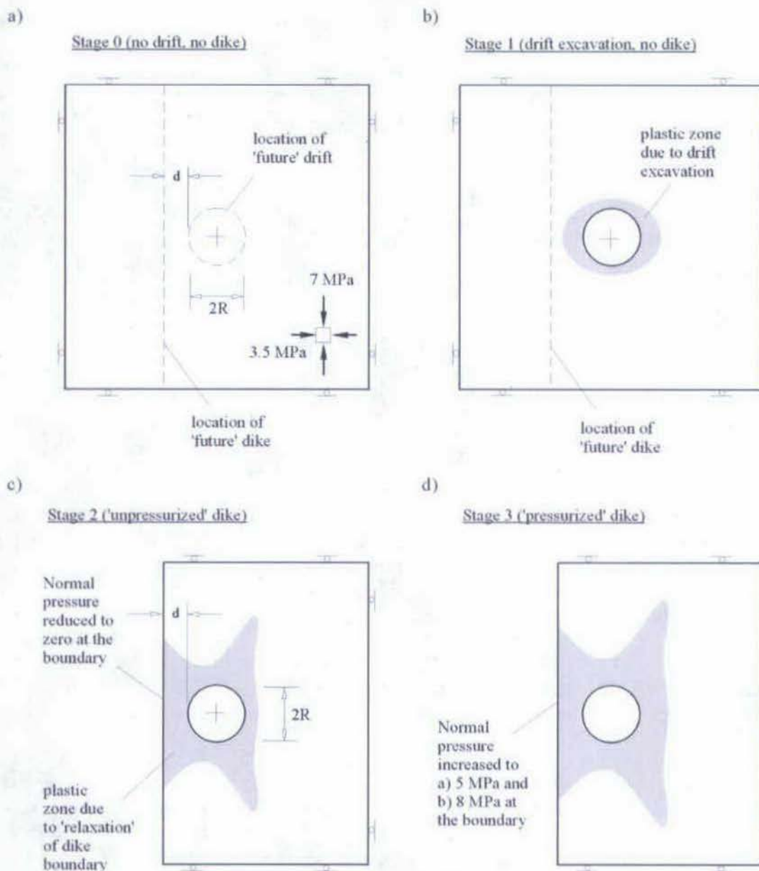
Figure G-2. Stages 0, 1, 2, and 3 Considered in the Calculation of Mechanical Interaction between Dike and Drift
