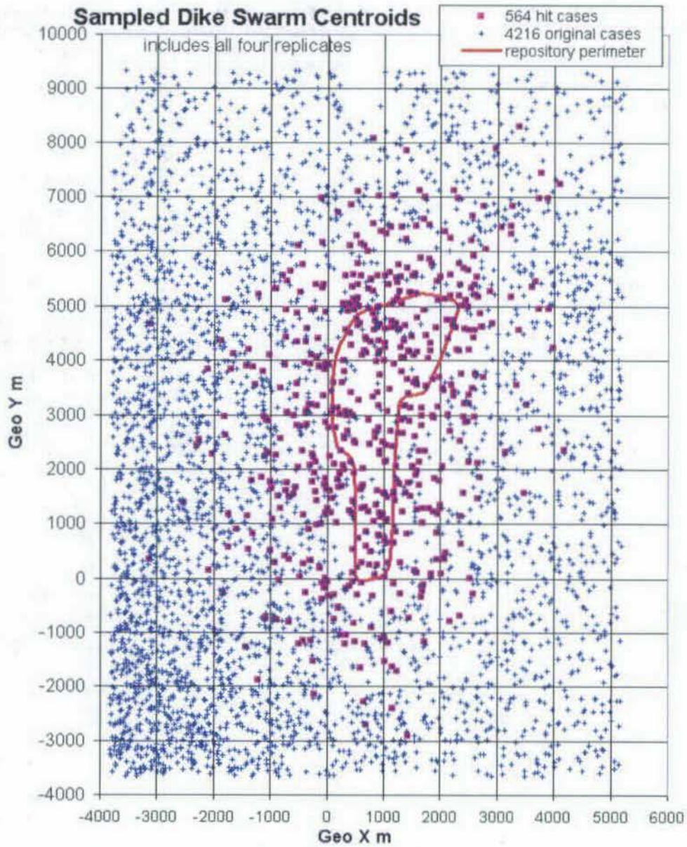
Figure 6-4. Sampled Dike Swarm Centroids
