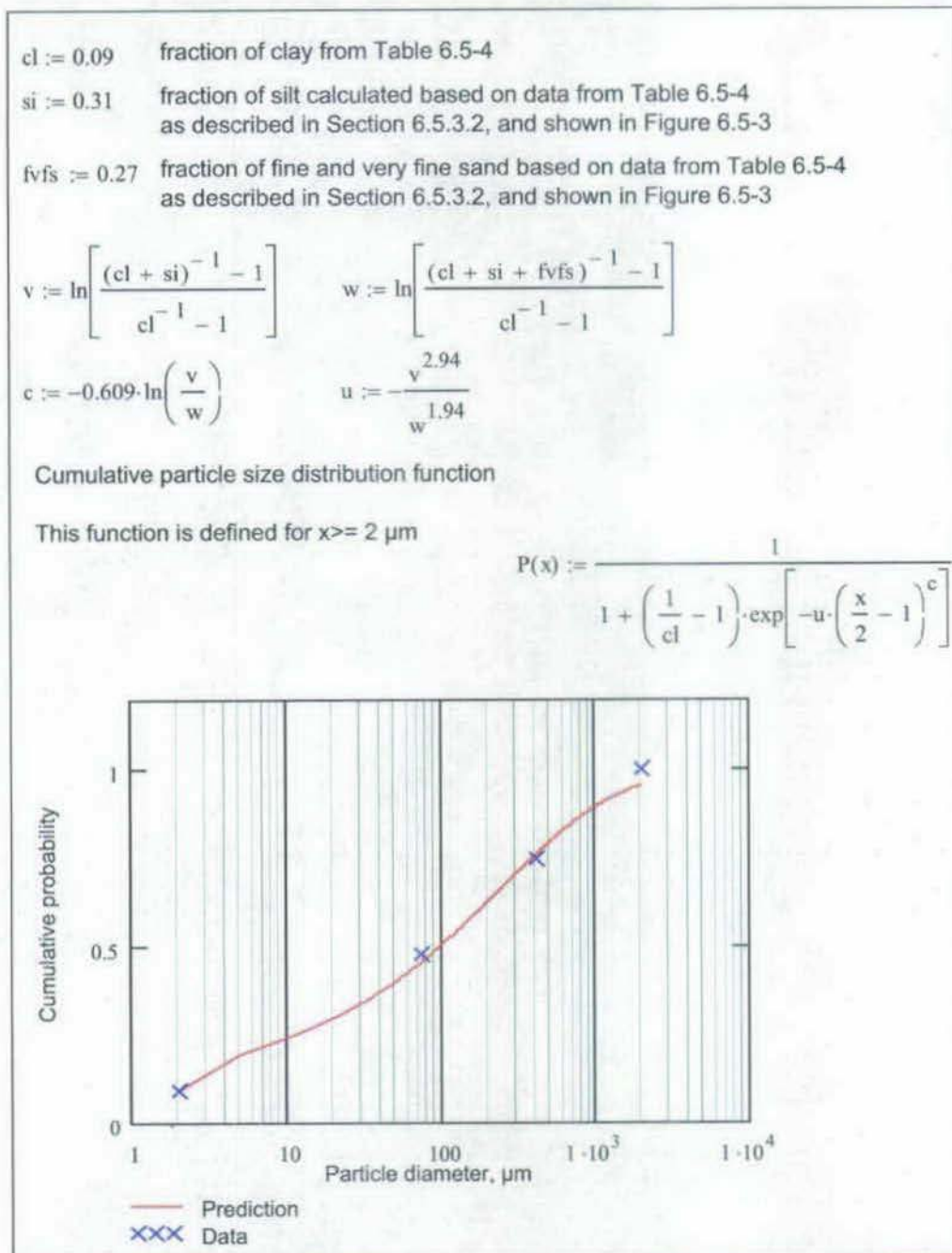
Figure 6.5-4. Cumulative Particle Size Distribution Function for Amargosa Valley Soils
