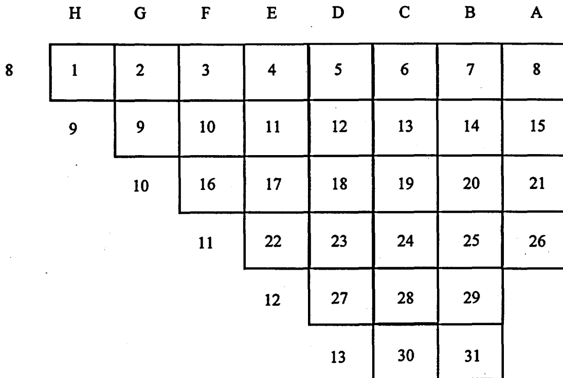
Figure 5.2.5-1. One-Eighth Symmetric Core Layout for Sequoyah Unit 2
