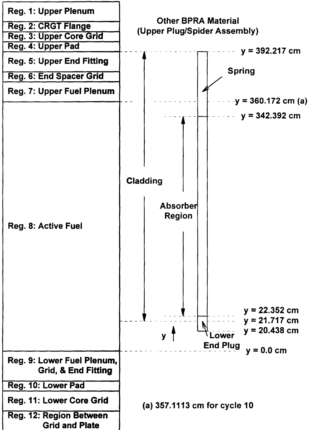
Figure 2-12. Axial Dimensions for BPRA
