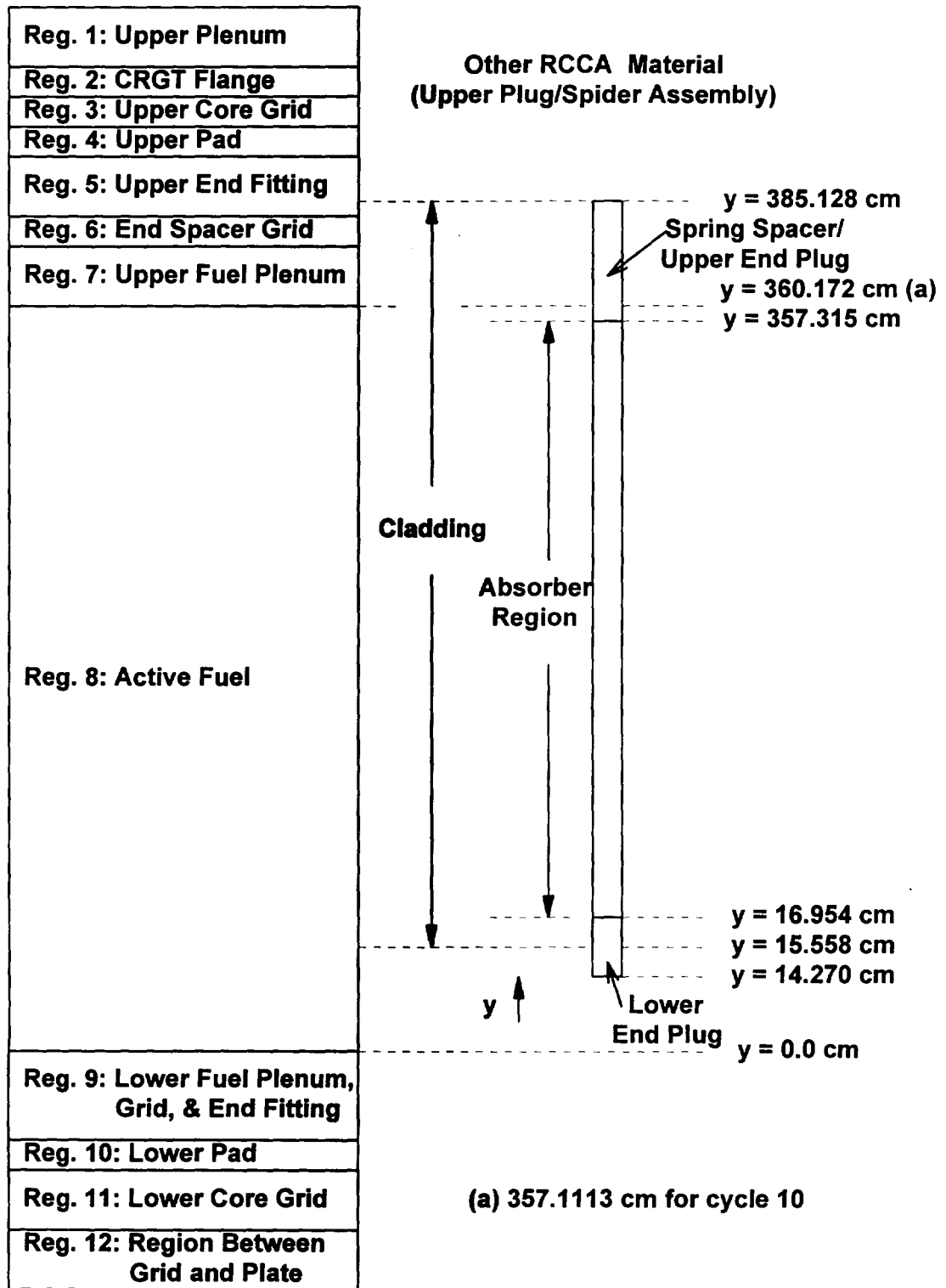
Figure 2-8. Axial Dimensions for RCCAs (0% Withdrawn)
