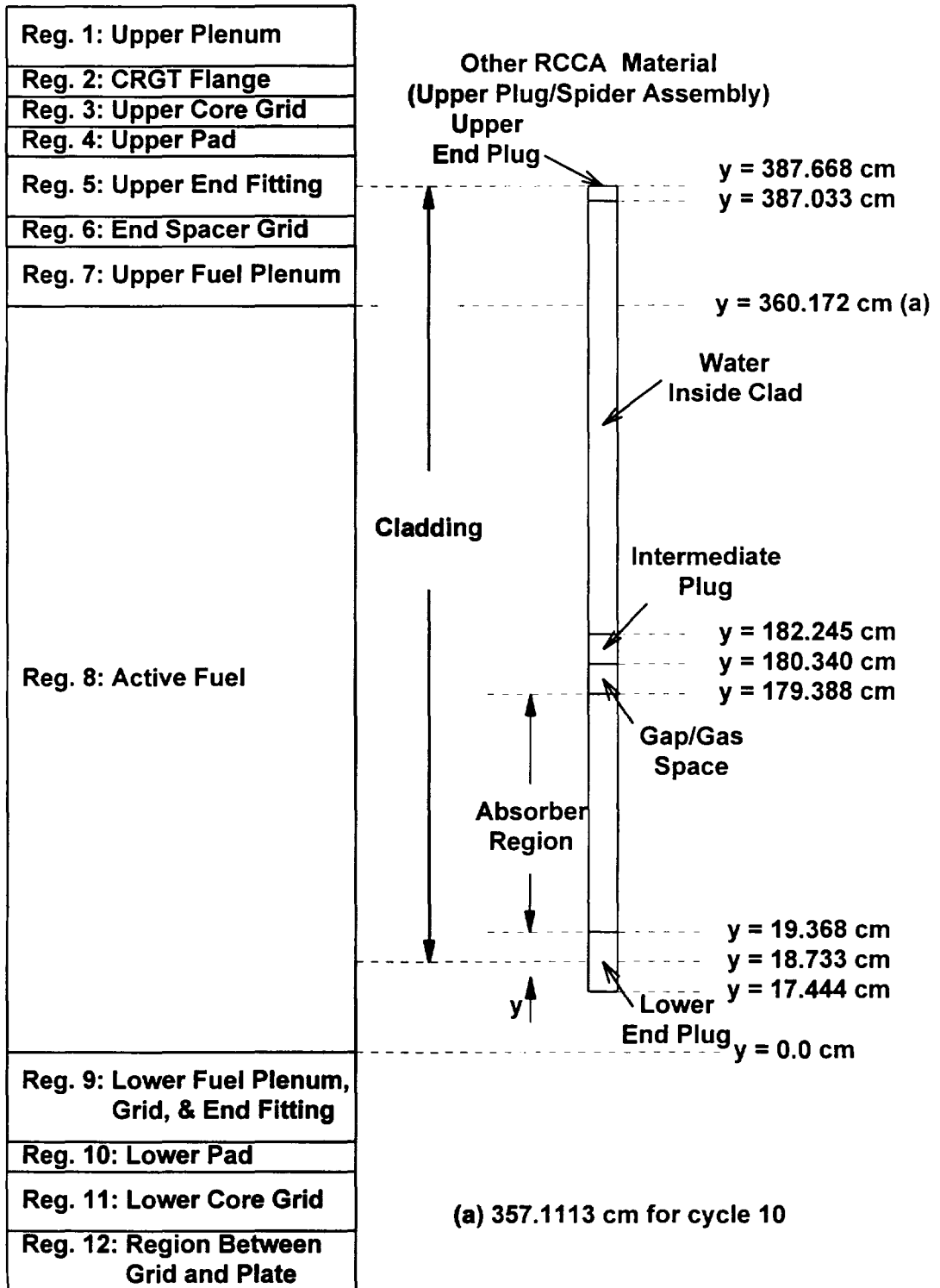
Figure 2-11. Axial Dimensions for Gray APSR (0% Withdrawn)
