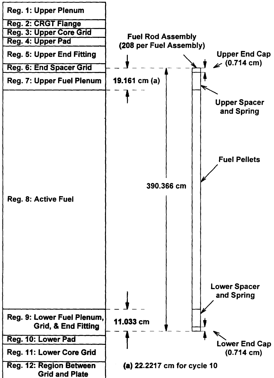
Figure 2-7. Axial Dimensions for Fuel Rod Assembly
