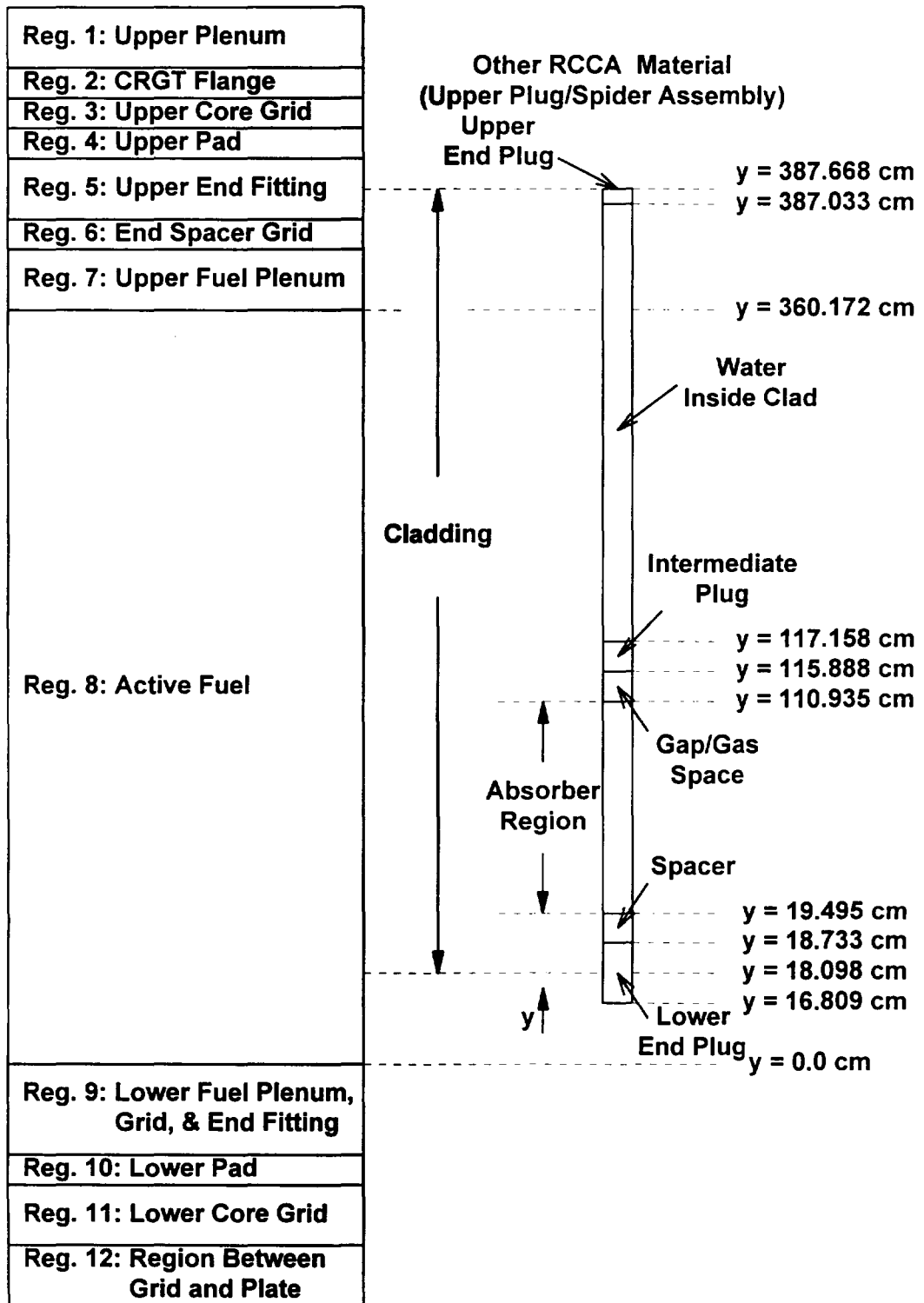
Figure 2-10. Axial Dimensions for Black APSR (0% Withdrawn)
