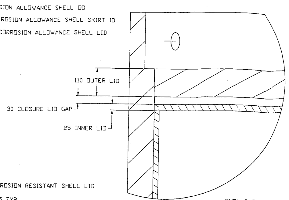
DETAIL A BASKET COMPONENTS NOT SHOWN IN THIS VIEW
