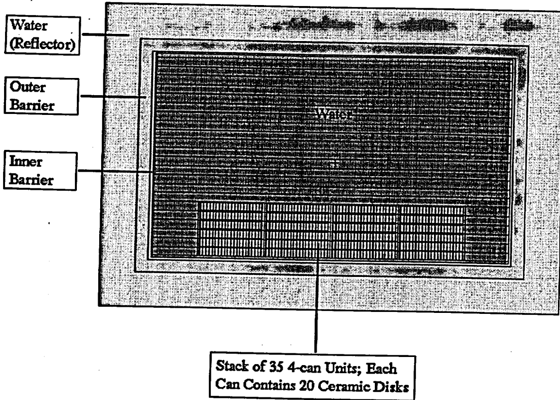
Figure 5.2.1.1-2. A Cross-sectional Side View of a Horizontally Emplaced Waste Package for the Square Lattice Arrangement of Cans in a "Square" Geometry
