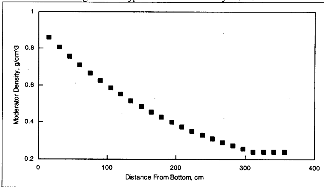
Figure 7-1. Typical Moderator Density Profile
