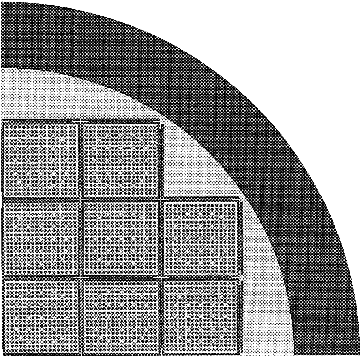
Figure 24 Cross-sectional view of one quarter of the KENO V.a calculational model of the GBC-32 cask loaded with Westinghouse 17 x 17 assemblies
