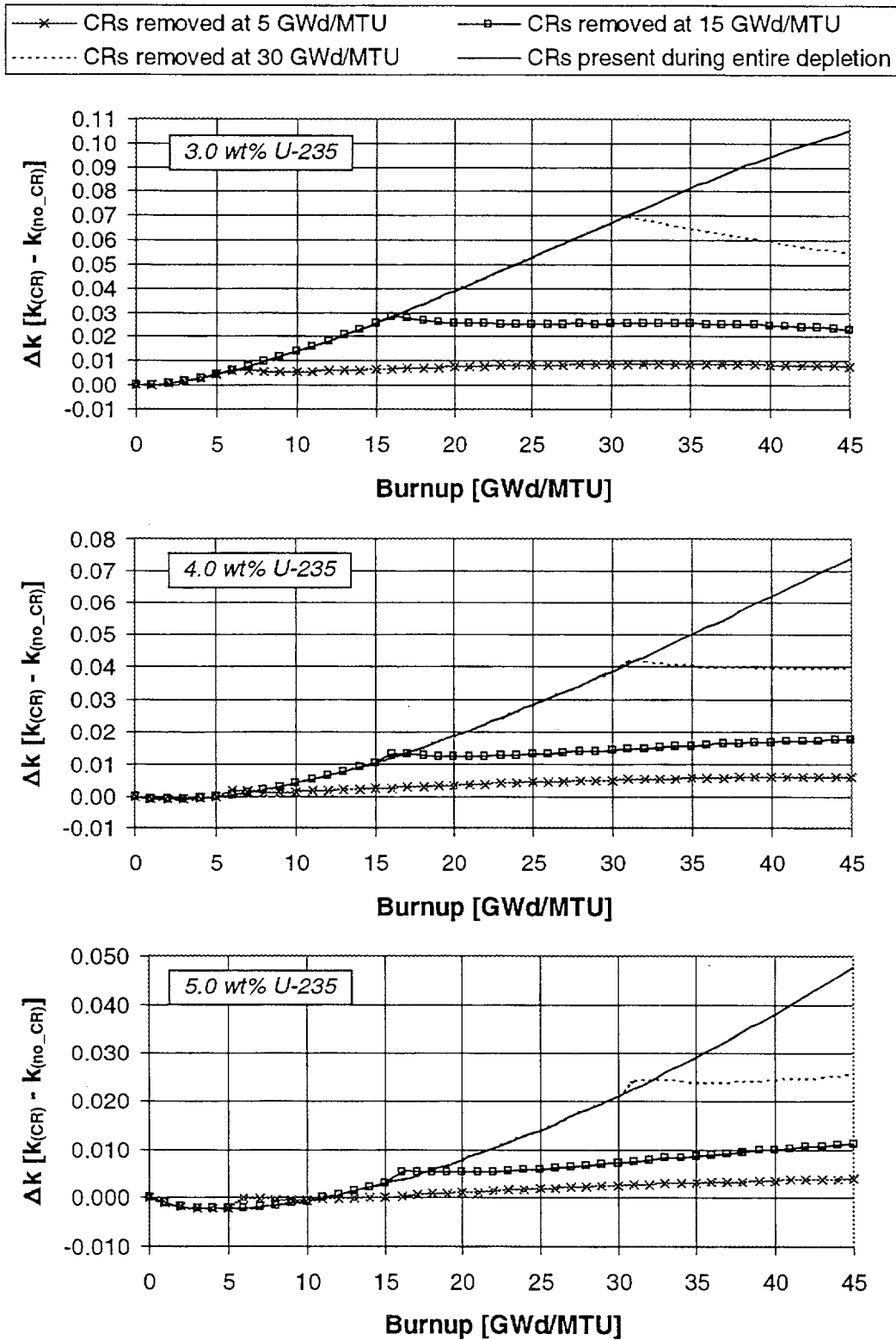
Figure 10 Comparison of \Delta k values as a function of burnup for various CR exposures with initial fuel enrichments of 3, 4, and 5 wt% ^{235}\text{U} . The results correspond to Westinghouse 17 \times 17 fuel and the \text{B}_4\text{C} axial segment of the hybrid Ag-In-Cd/ \text{B}_4\text{C} CRs.
