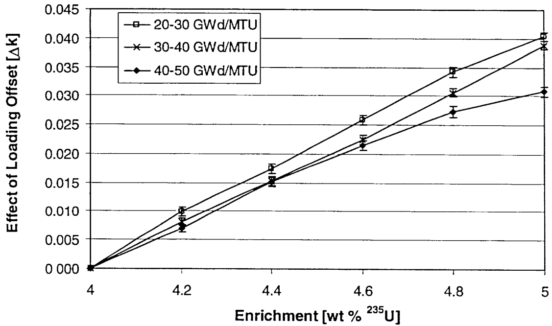
Figure 32 Effect of the loading offset for actinide-only burnup credit
