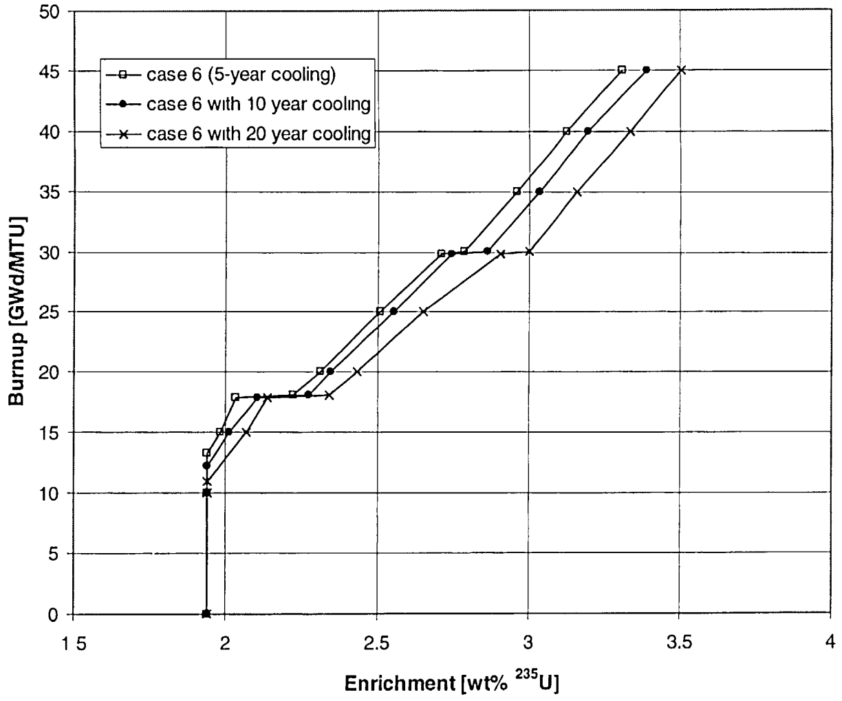
Figure 40 Effect of cooling time on loading curves for actinide-only burnup credit (see Table 10 for specification of case 6)
