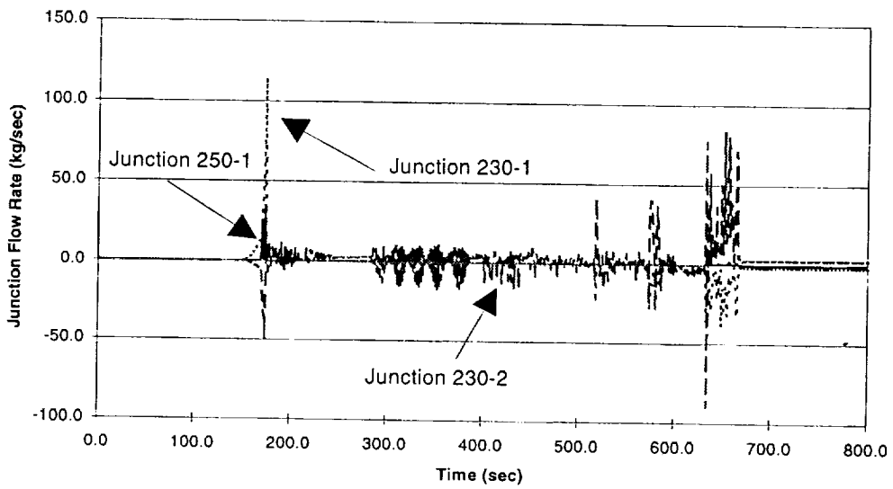
Figure 8.4-16. Junction Flow Rates - 3,600 second Reactivity Insertion Scenario
