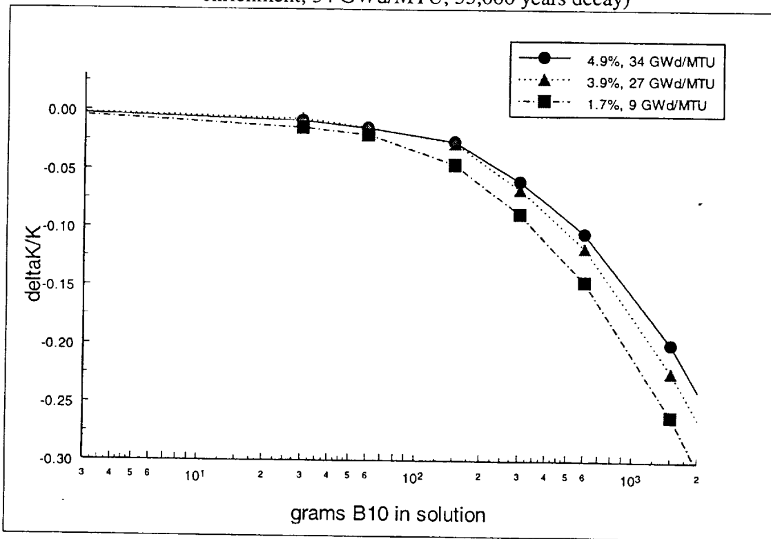
Figure 6.2.2-6. Effects of dissolved ^{10}\text{B} on fully degraded basket k_{eff} for the 58 vol% settled oxide configuration
