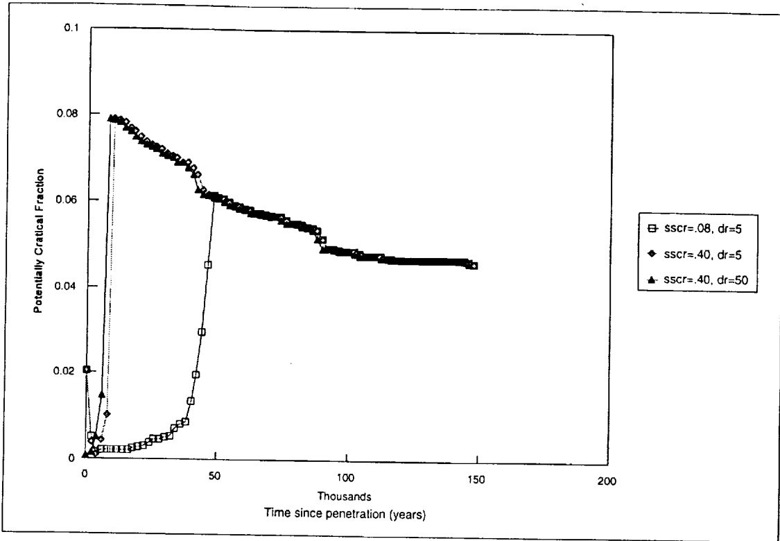
Figure 7.3-1. Time Dependence of Potentially Critical Fraction - Settled Oxide, WP Penetration Time = 3,000 years
