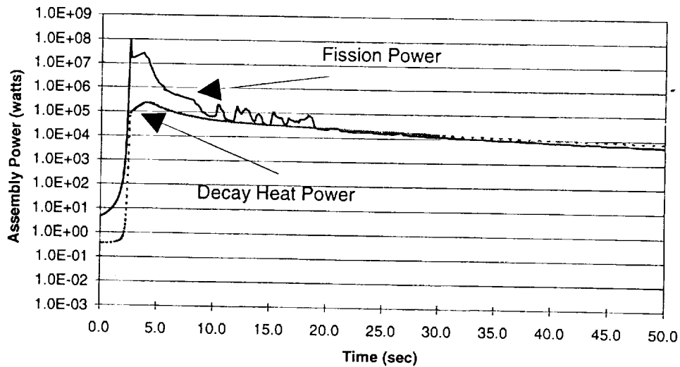
Figure 8.4-2. Assembly Power - 30 second Reactivity Insertion Scenario
