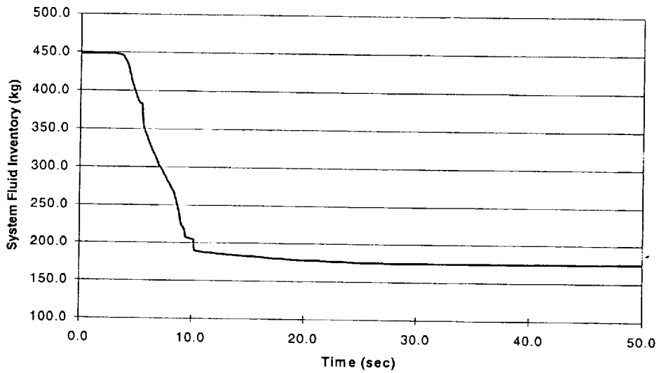
Figure 8.4-6. Waste Package Fluid Inventory - 30 second Reactivity Insertion Scenario
