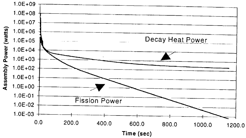
Figure 8.4-1. Assembly Power - 30 second Reactivity Insertion Scenario
