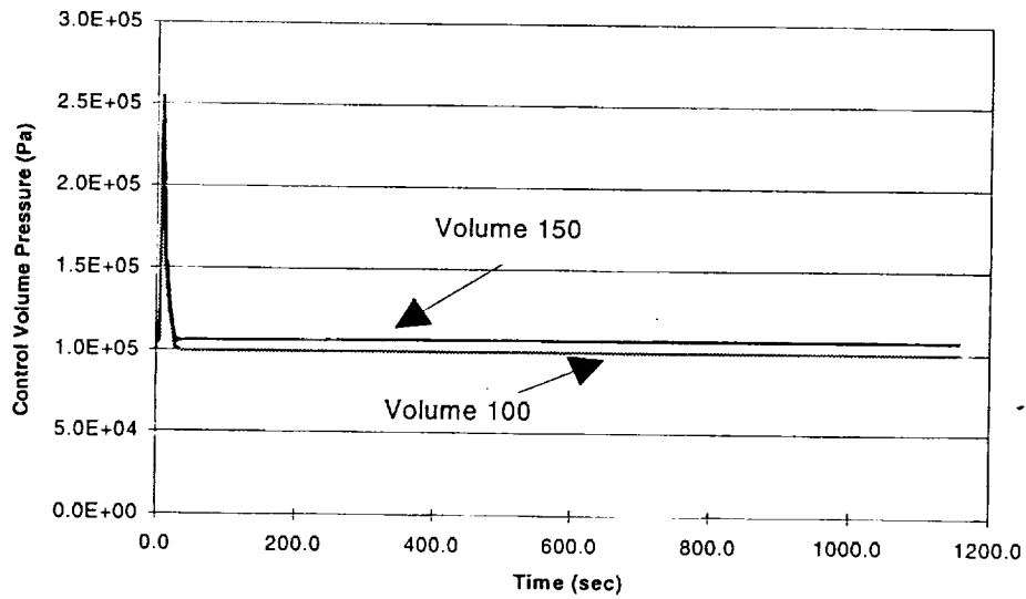
Figure 8.4-4. Volume Pressures - 30 second Reactivity Insertion Scenario
