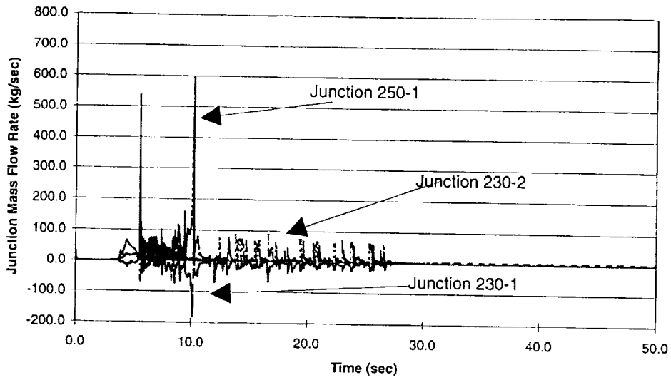
Figure 8.4-7. Junction Flow Rates - 30 second Reactivity Insertion Scenario
