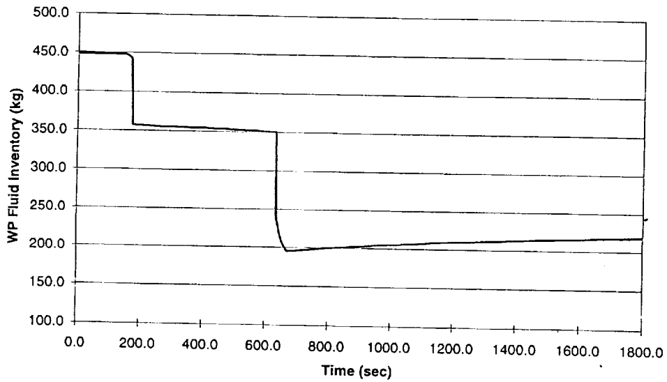
Figure 8.4-12. Waste Package Fluid Inventory - 3,600 second Reactivity Insertion Scenario
