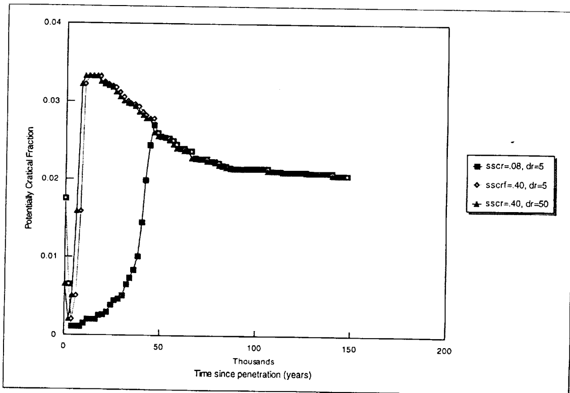
Figure 7.3-2. Time Dependence of Potentially Critical Fraction - Uniform Oxide, WP Penetration Time = 3,000 years
