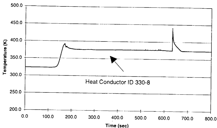
Figure 8.4-17. Average Metal Temperature* - 3,600 second Reactivity Insertion Scenario
