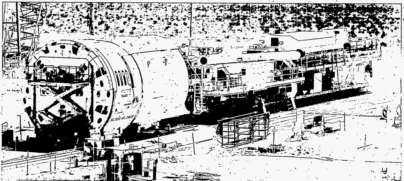
The center cutter section of the TBM (A) winds its way down US-95 through Indian Springs, Nevada, en route to the TBM assembly pad at Yucca Mountain. Upon arrival (B&C), the TBM parts were uncrated, assembled and tested.
